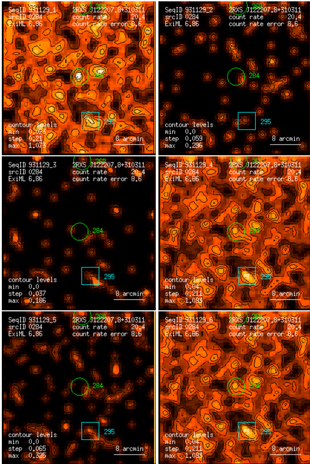
Figure 284: RASS 931129: detection 0284: band rate images, Gaussian filter: (1) PSPC channels 11 – 41, (2) 52 – 90, (3) 91 – 201, (4) 11 – 235, (5) 52 – 201, (6) 11 – 201. Broad band rates in counts/ks. Band rate contour levels in counts/ks/arcmin 2 .
