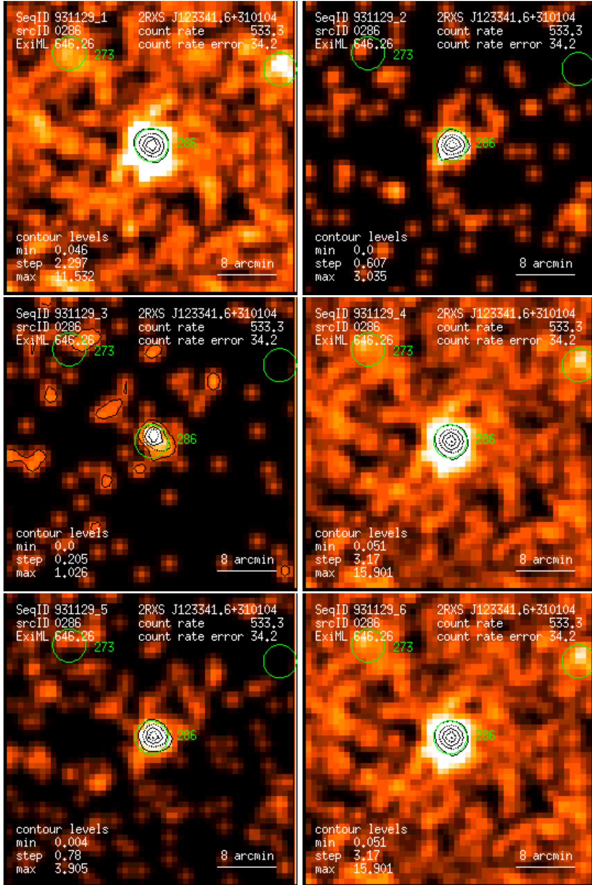
Figure 286: RASS 931129: detection 0286: band rate images, Gaussian filter: (1) PSPC channels 11 – 41, (2) 52 – 90, (3) 91 – 201, (4) 11 – 235, (5) 52 – 201, (6) 11 – 201. Broad band rates in counts/ks. Band rate contour levels in counts/ks/arcmin 2 .
