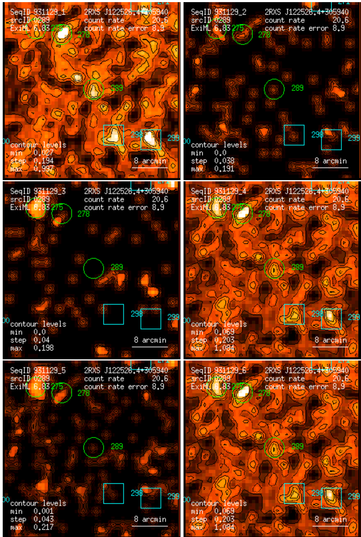
Figure 289: RASS 931129: detection 0289: band rate images, Gaussian filter: (1) PSPC channels 11 – 41, (2) 52 – 90, (3) 91 – 201, (4) 11 – 235, (5) 52 – 201, (6) 11 – 201. Broad band rates in counts/ks. Band rate contour levels in counts/ks/arcmin 2 .
