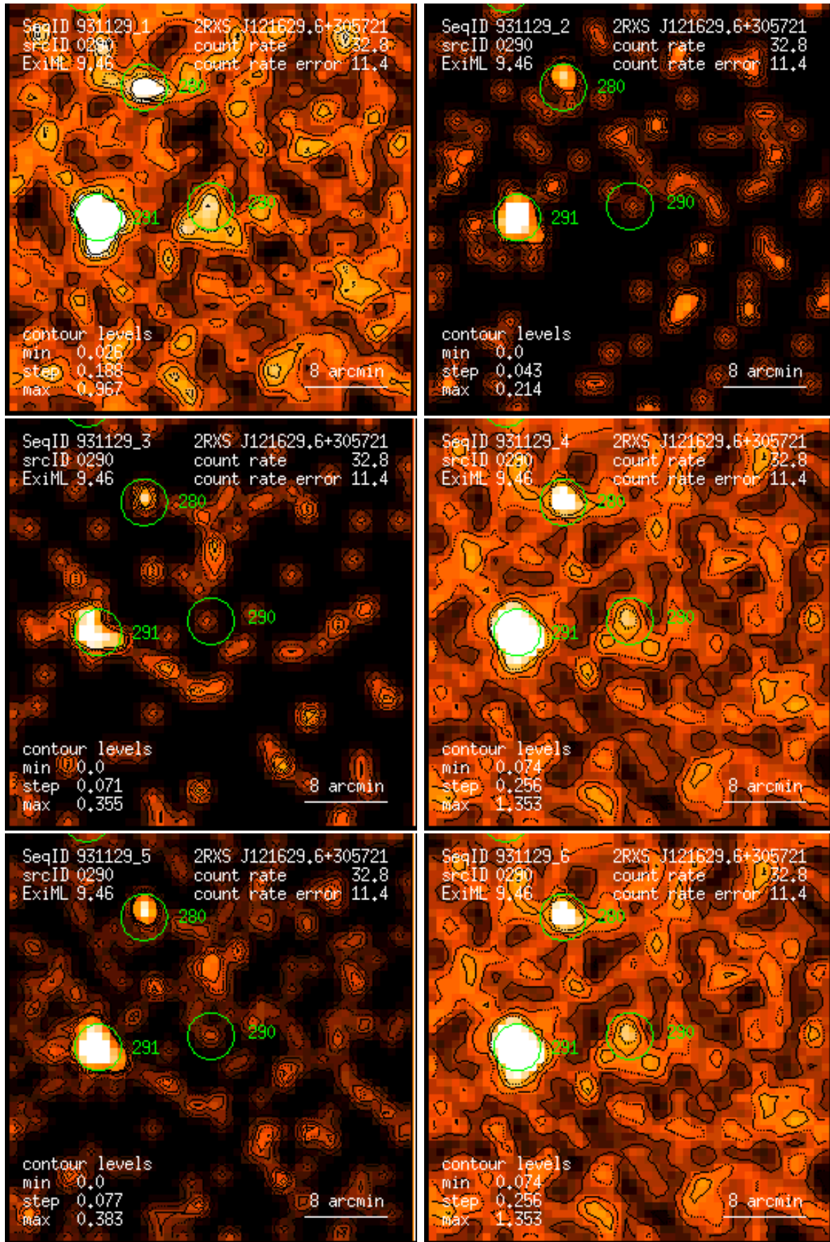
Figure 290: RASS 931129: detection 0290: band rate images, Gaussian filter: (1) PSPC channels 11 – 41, (2) 52 – 90, (3) 91 – 201, (4) 11 – 235, (5) 52 – 201, (6) 11 – 201. Broad band rates in counts/ks. Band rate contour levels in counts/ks/arcmin 2 .
