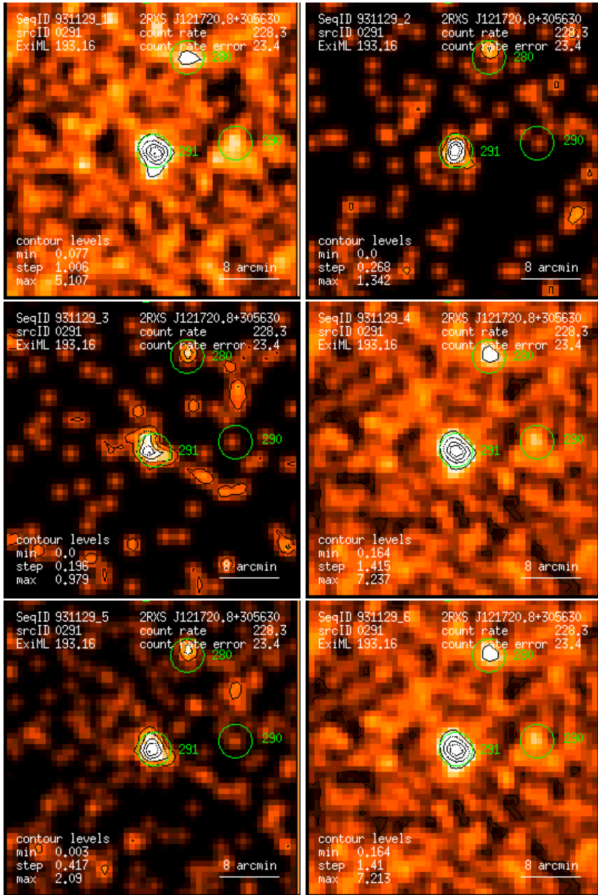
Figure 291: RASS 931129: detection 0291: band rate images, Gaussian filter: (1) PSPC channels 11 – 41, (2) 52 – 90, (3) 91 – 201, (4) 11 – 235, (5) 52 – 201, (6) 11 – 201. Broad band rates in counts/ks. Band rate contour levels in counts/ks/arcmin 2 .
