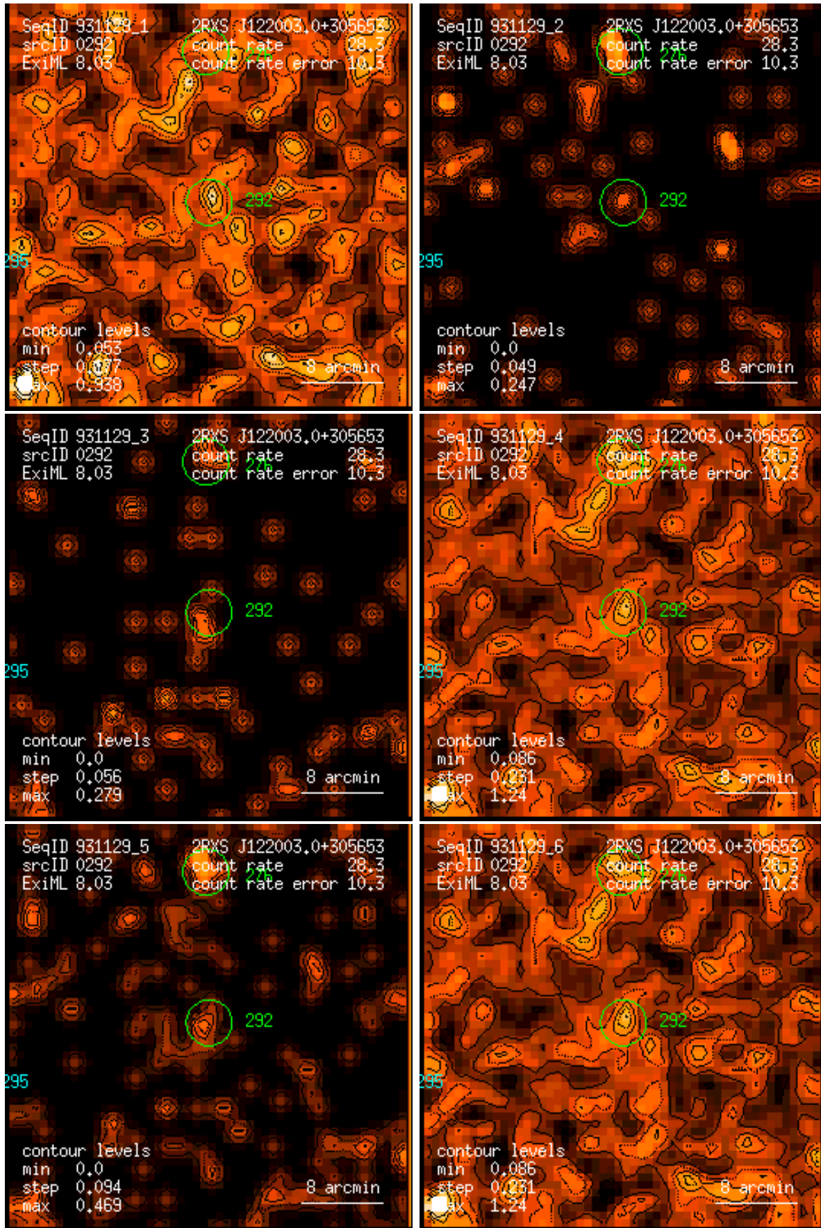
Figure 292: RASS 931129: detection 0292: band rate images, Gaussian filter: (1) PSPC channels 11 – 41, (2) 52 – 90, (3) 91 – 201, (4) 11 – 235, (5) 52 – 201, (6) 11 – 201. Broad band rates in counts/ks. Band rate contour levels in counts/ks/arcmin 2 .
