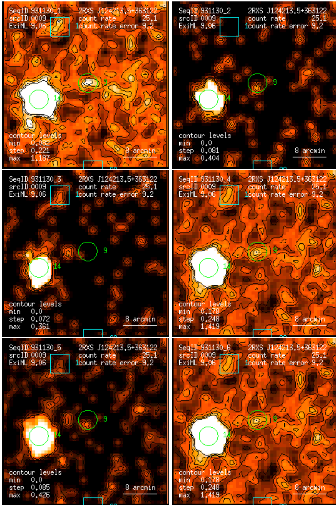
Figure 9: RASS 931130: detection 0009: band rate images, Gaussian filter: (1) PSPC channels 11 – 41, (2) 52 – 90, (3) 91 – 201, (4) 11 – 235, (5) 52 – 201, (6) 11 – 201. Broad band rates in counts/ks. Band rate contour levels in counts/ks/arcmin 2 .
