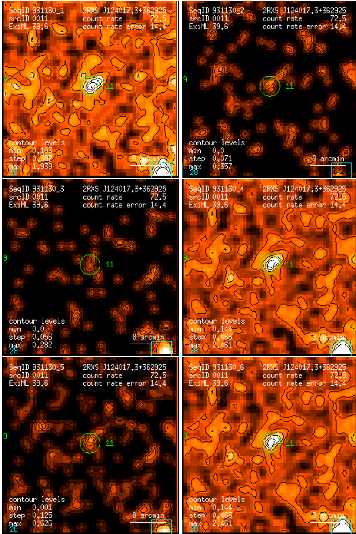
Figure 11: RASS 931130: detection 0011: band rate images, Gaussian filter: (1) PSPC channels 11 – 41, (2) 52 – 90, (3) 91 – 201, (4) 11 – 235, (5) 52 – 201, (6) 11 – 201. Broad band rates in counts/ks. Band rate contour levels in counts/ks/arcmin 2 .
