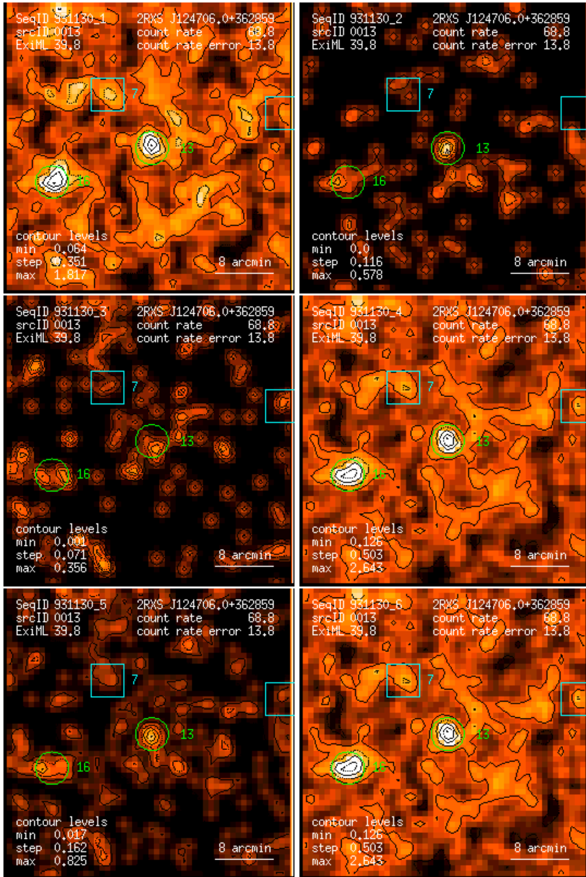
Figure 13: RASS 931130: detection 0013: band rate images, Gaussian filter: (1) PSPC channels 11 – 41, (2) 52 – 90, (3) 91 – 201, (4) 11 – 235, (5) 52 – 201, (6) 11 – 201. Broad band rates in counts/ks. Band rate contour levels in counts/ks/arcmin 2 .
