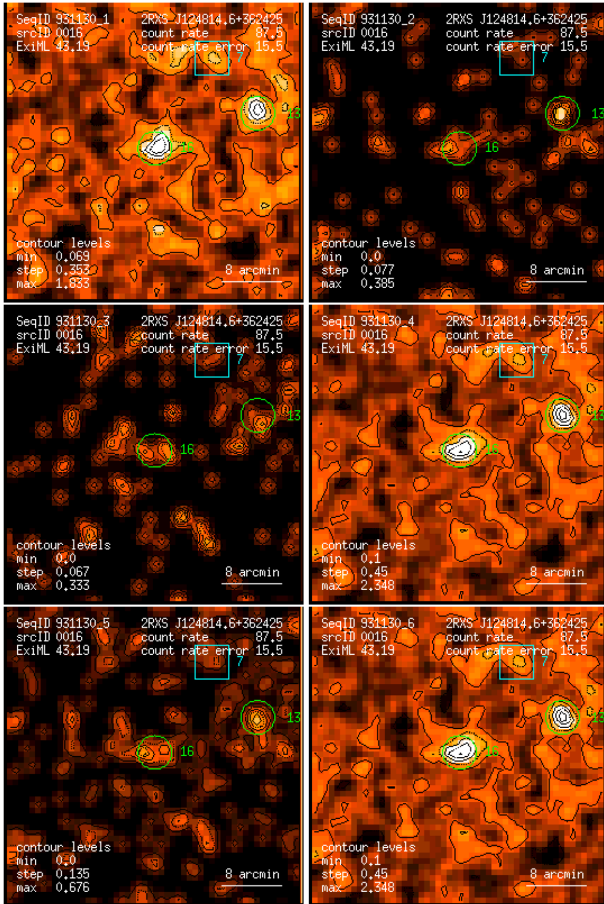
Figure 16: RASS 931130: detection 0016: band rate images, Gaussian filter: (1) PSPC channels 11 – 41, (2) 52 – 90, (3) 91 – 201, (4) 11 – 235, (5) 52 – 201, (6) 11 – 201. Broad band rates in counts/ks. Band rate contour levels in counts/ks/arcmin 2 .
