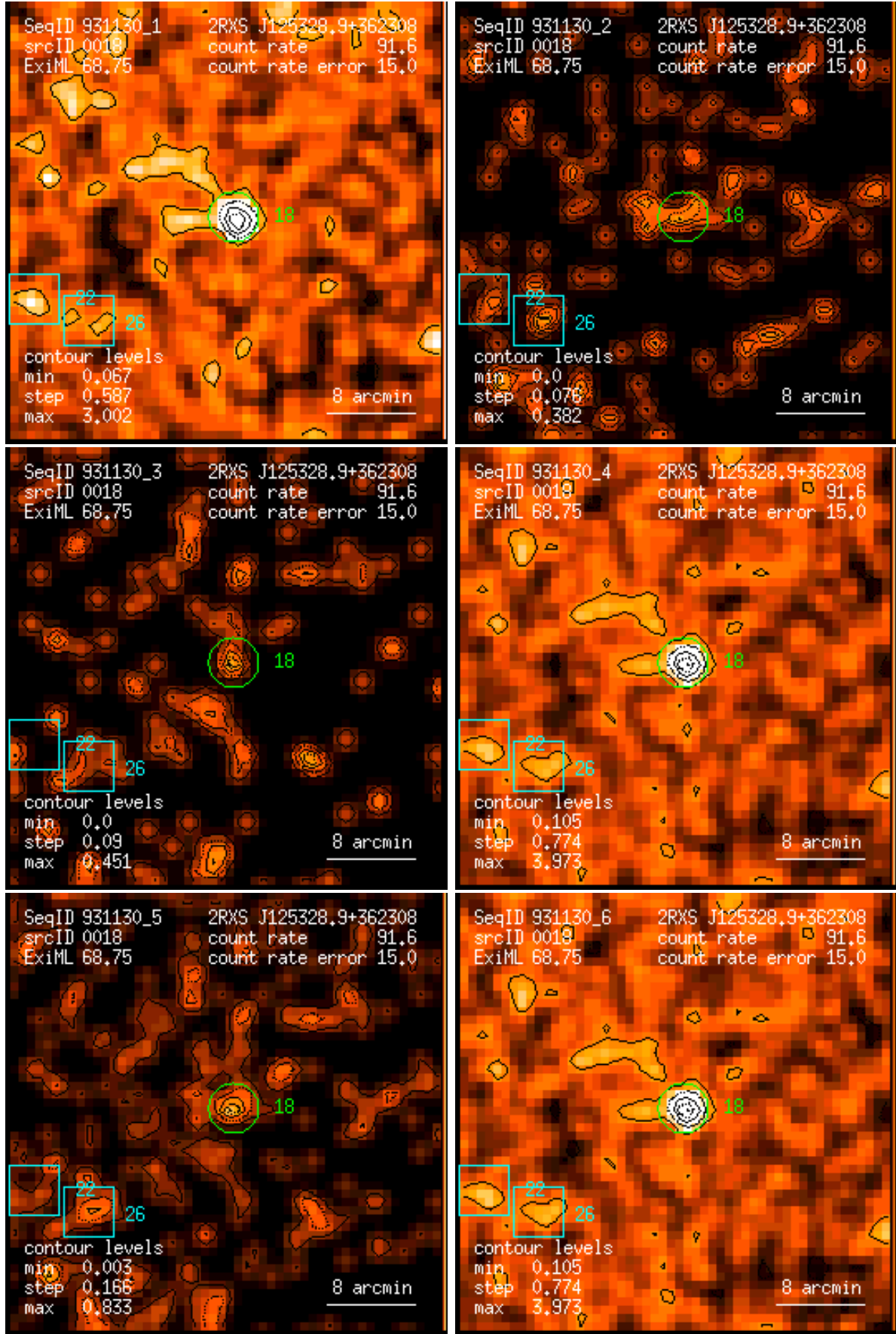
Figure 18: RASS 931130: detection 0018: band rate images, Gaussian filter: (1) PSPC channels 11 – 41, (2) 52 – 90, (3) 91 – 201, (4) 11 – 235, (5) 52 – 201, (6) 11 – 201. Broad band rates in counts/ks. Band rate contour levels in counts/ks/arcmin 2 .
