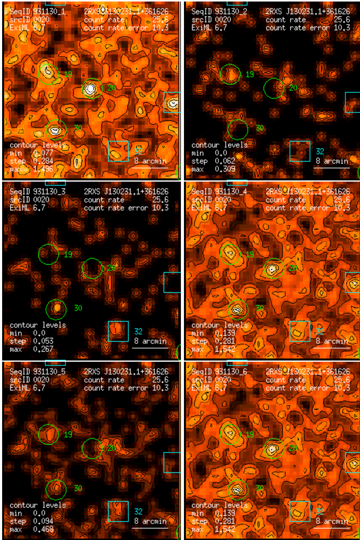
Figure 20: RASS 931130: detection 0020: band rate images, Gaussian filter: (1) PSPC channels 11 – 41, (2) 52 – 90, (3) 91 – 201, (4) 11 – 235, (5) 52 – 201, (6) 11 – 201. Broad band rates in counts/ks. Band rate contour levels in counts/ks/arcmin 2 .
