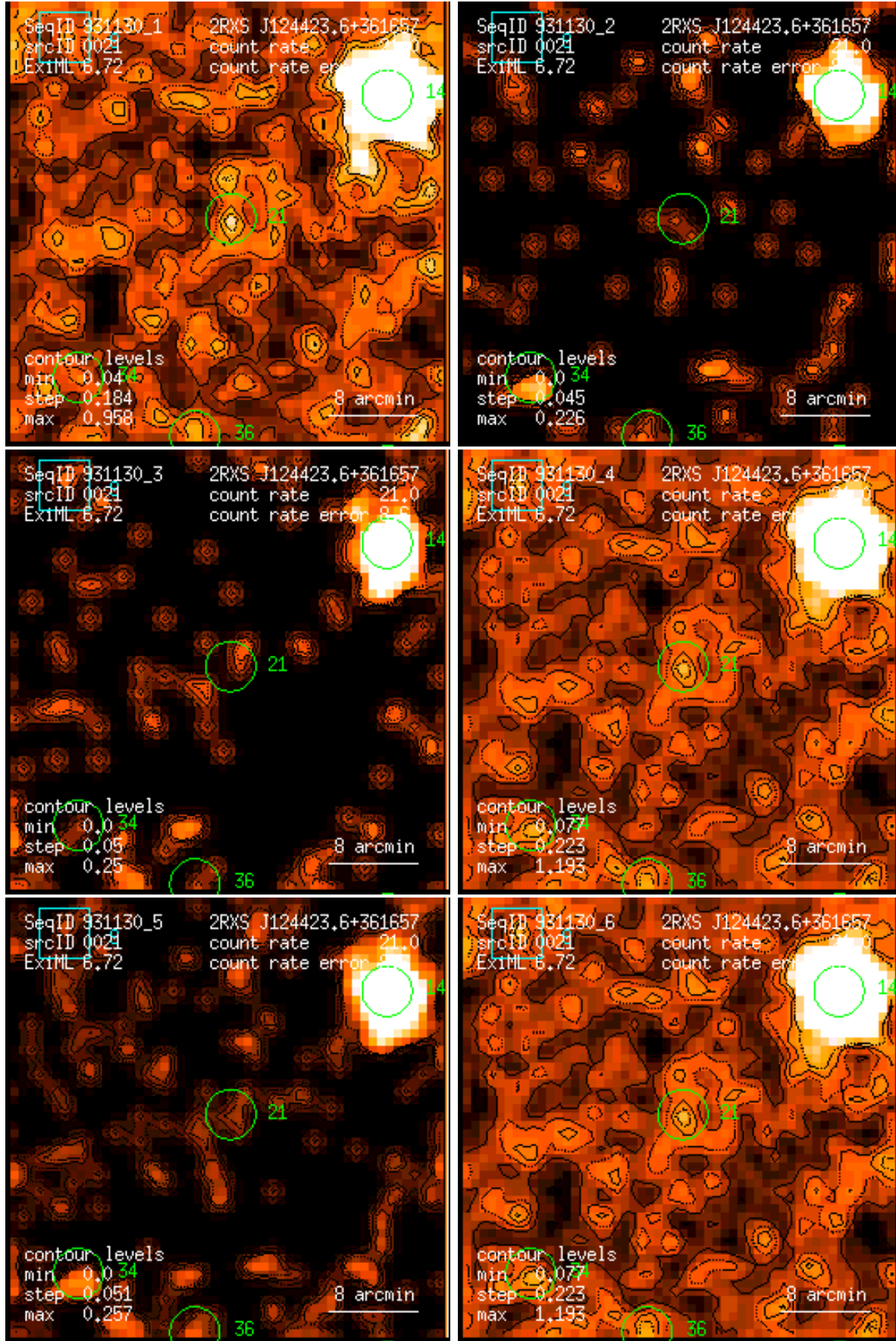
Figure 21: RASS 931130: detection 0021: band rate images, Gaussian filter: (1) PSPC channels 11 – 41, (2) 52 – 90, (3) 91 – 201, (4) 11 – 235, (5) 52 – 201, (6) 11 – 201. Broad band rates in counts/ks. Band rate contour levels in counts/ks/arcmin 2 .
