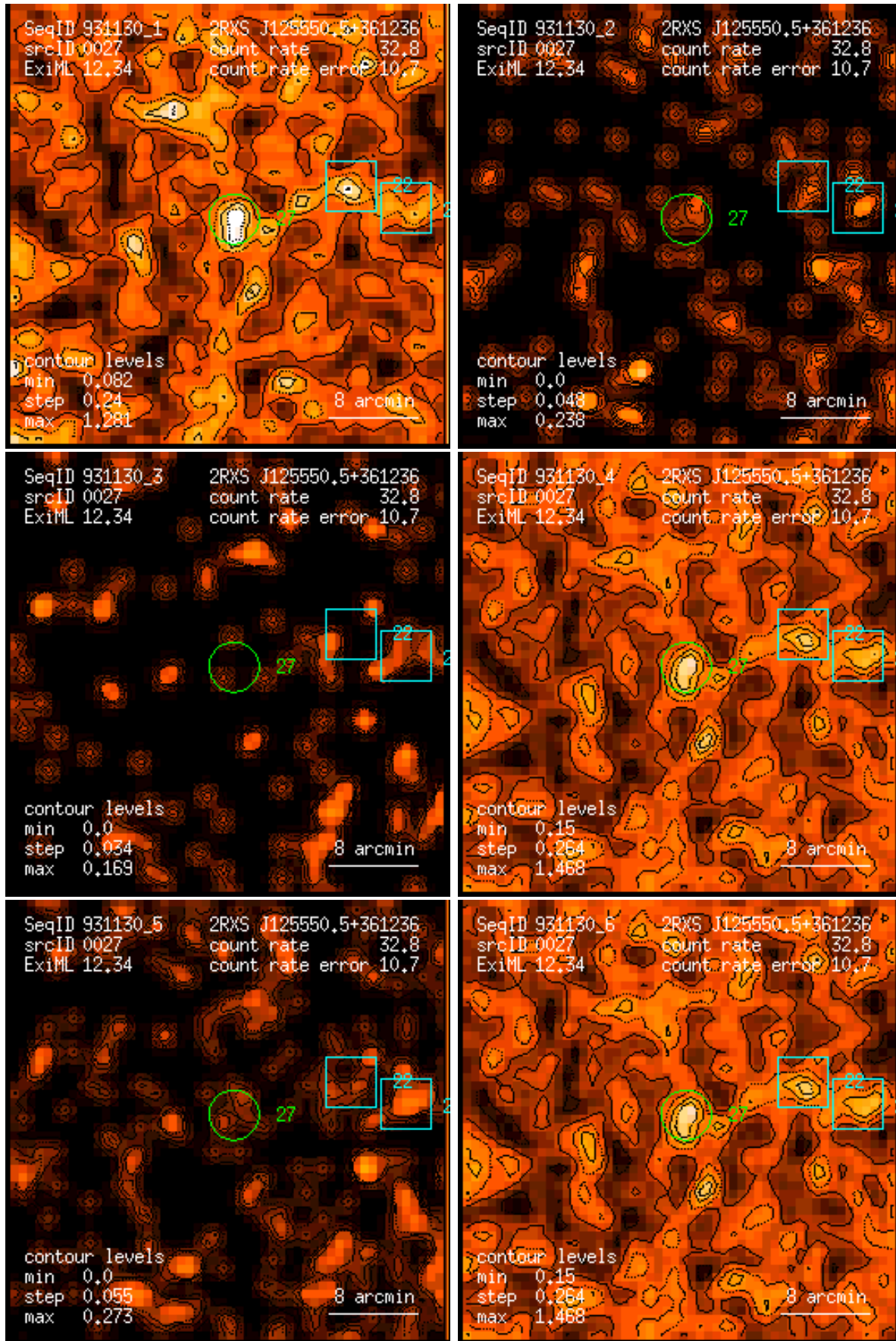
Figure 27: RASS 931130: detection 0027: band rate images, Gaussian filter: (1) PSPC channels 11 – 41, (2) 52 – 90, (3) 91 – 201, (4) 11 – 235, (5) 52 – 201, (6) 11 – 201. Broad band rates in counts/ks. Band rate contour levels in counts/ks/arcmin 2 .
