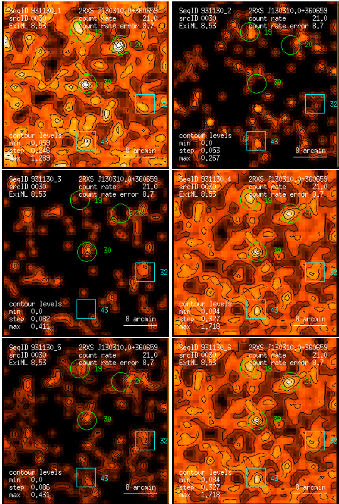
Figure 30: RASS 931130: detection 0030: band rate images, Gaussian filter: (1) PSPC channels 11 – 41, (2) 52 – 90, (3) 91 – 201, (4) 11 – 235, (5) 52 – 201, (6) 11 – 201. Broad band rates in counts/ks. Band rate contour levels in counts/ks/arcmin 2 .
