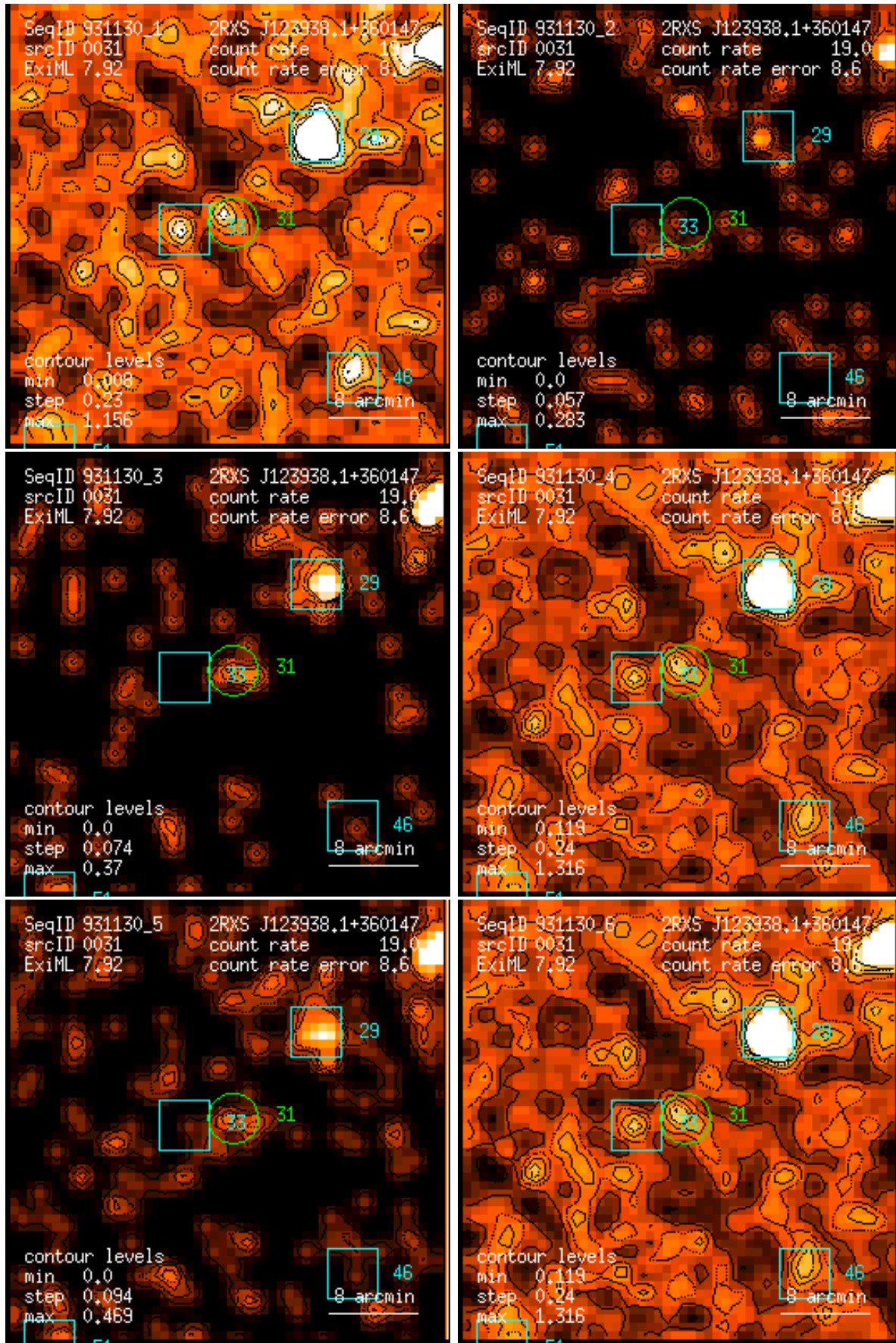
Figure 31: RASS 931130: detection 0031: band rate images, Gaussian filter: (1) PSPC channels 11 – 41, (2) 52 – 90, (3) 91 – 201, (4) 11 – 235, (5) 52 – 201, (6) 11 – 201. Broad band rates in counts/ks. Band rate contour levels in counts/ks/arcmin 2 .
