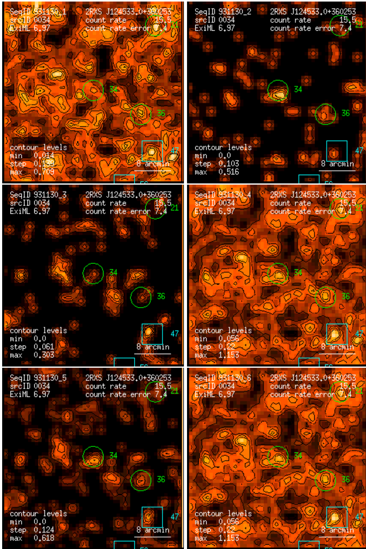
Figure 34: RASS 931130: detection 0034: band rate images, Gaussian filter: (1) PSPC channels 11 – 41, (2) 52 – 90, (3) 91 – 201, (4) 11 – 235, (5) 52 – 201, (6) 11 – 201. Broad band rates in counts/ks. Band rate contour levels in counts/ks/arcmin 2 .
