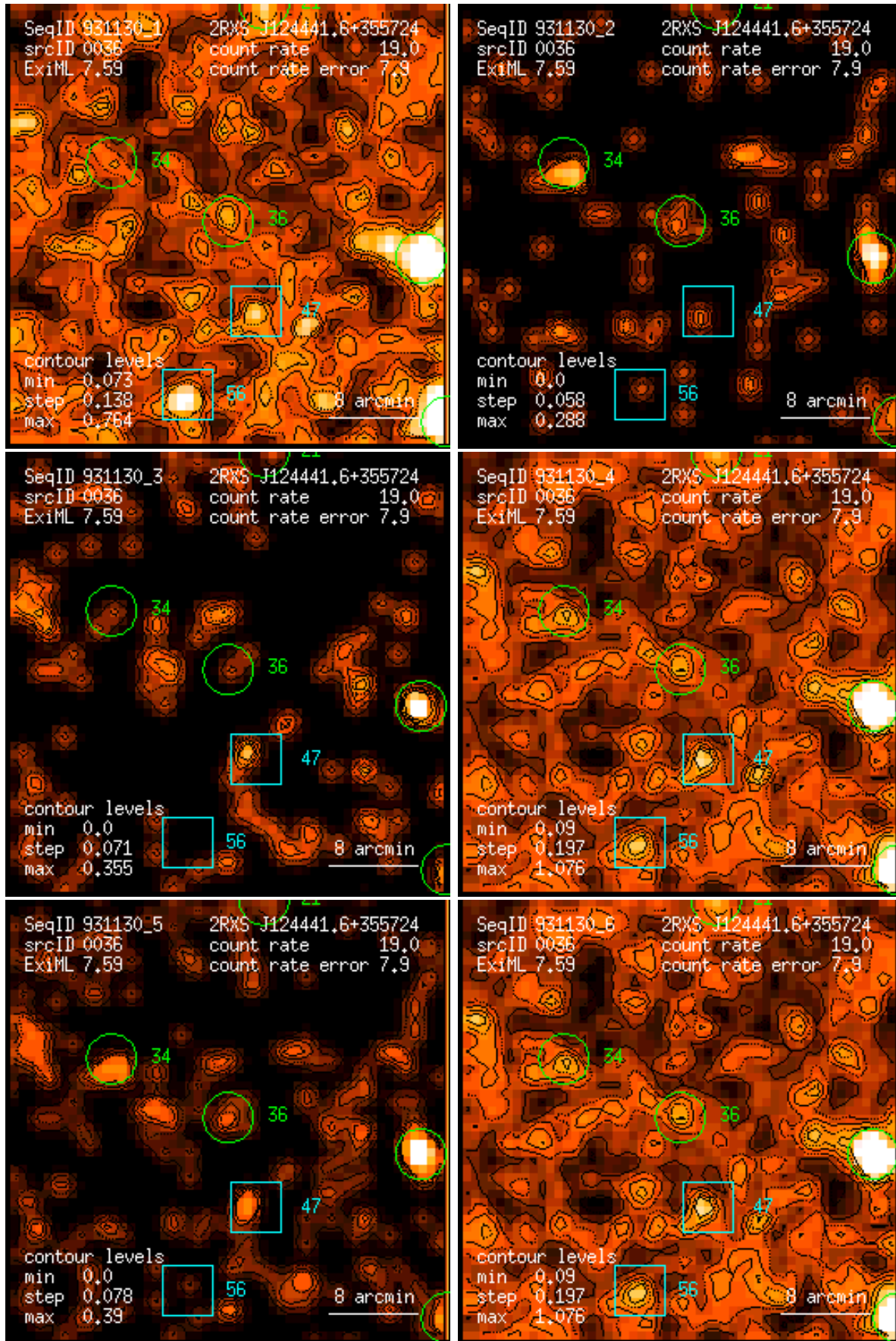
Figure 36: RASS 931130: detection 0036: band rate images, Gaussian filter: (1) PSPC channels 11 – 41, (2) 52 – 90, (3) 91 – 201, (4) 11 – 235, (5) 52 – 201, (6) 11 – 201. Broad band rates in counts/ks. Band rate contour levels in counts/ks/arcmin 2 .
