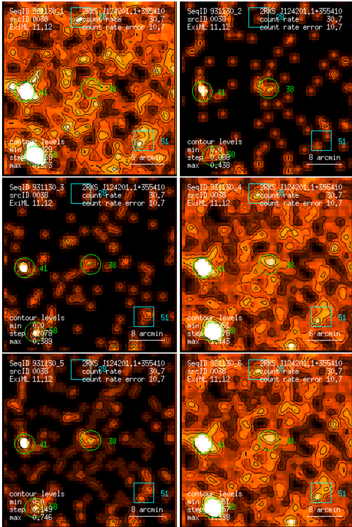
Figure 38: RASS 931130: detection 0038: band rate images, Gaussian filter: (1) PSPC channels 11 – 41, (2) 52 – 90, (3) 91 – 201, (4) 11 – 235, (5) 52 – 201, (6) 11 – 201. Broad band rates in counts/ks. Band rate contour levels in counts/ks/arcmin 2 .
