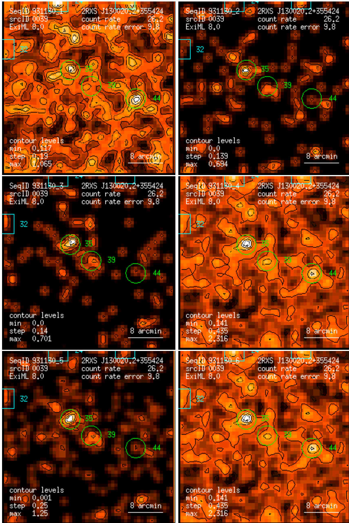
Figure 39: RASS 931130: detection 0039: band rate images, Gaussian filter: (1) PSPC channels 11 – 41, (2) 52 – 90, (3) 91 – 201, (4) 11 – 235, (5) 52 – 201, (6) 11 – 201. Broad band rates in counts/ks. Band rate contour levels in counts/ks/arcmin 2 .
