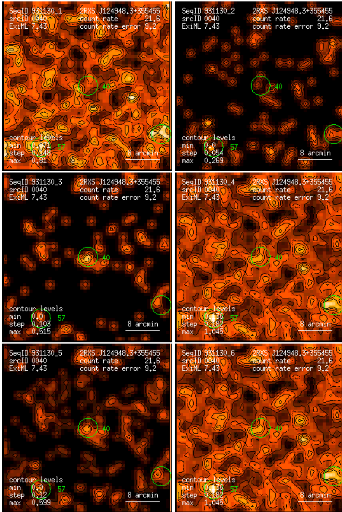
Figure 40: RASS 931130: detection 0040: band rate images, Gaussian filter: (1) PSPC channels 11 – 41, (2) 52 – 90, (3) 91 – 201, (4) 11 – 235, (5) 52 – 201, (6) 11 – 201. Broad band rates in counts/ks. Band rate contour levels in counts/ks/arcmin 2 .
