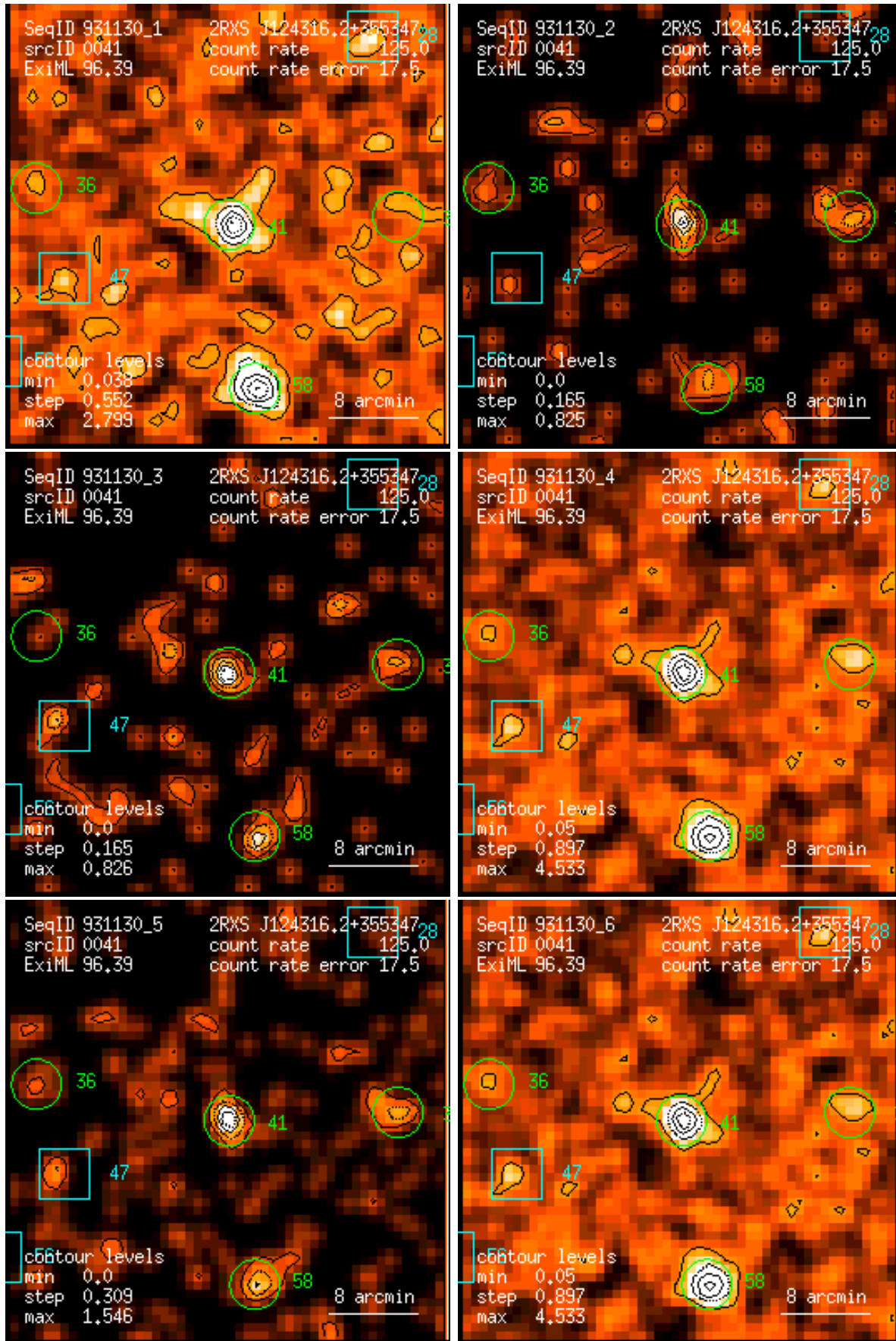
Figure 41: RASS 931130: detection 0041: band rate images, Gaussian filter: (1) PSPC channels 11 – 41, (2) 52 – 90, (3) 91 – 201, (4) 11 – 235, (5) 52 – 201, (6) 11 – 201. Broad band rates in counts/ks. Band rate contour levels in counts/ks/arcmin 2 .
