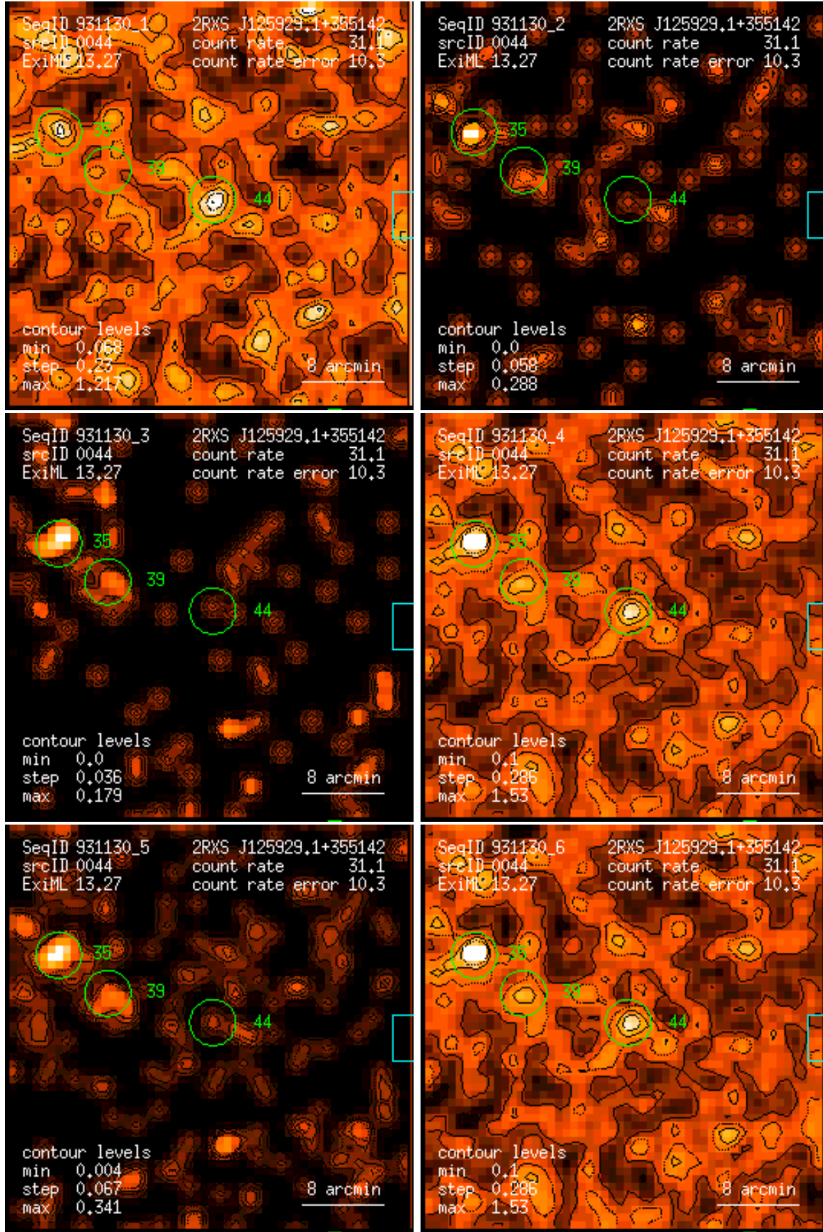
Figure 44: RASS 931130: detection 0044: band rate images, Gaussian filter: (1) PSPC channels 11 – 41, (2) 52 – 90, (3) 91 – 201, (4) 11 – 235, (5) 52 – 201, (6) 11 – 201. Broad band rates in counts/ks. Band rate contour levels in counts/ks/arcmin 2 .
