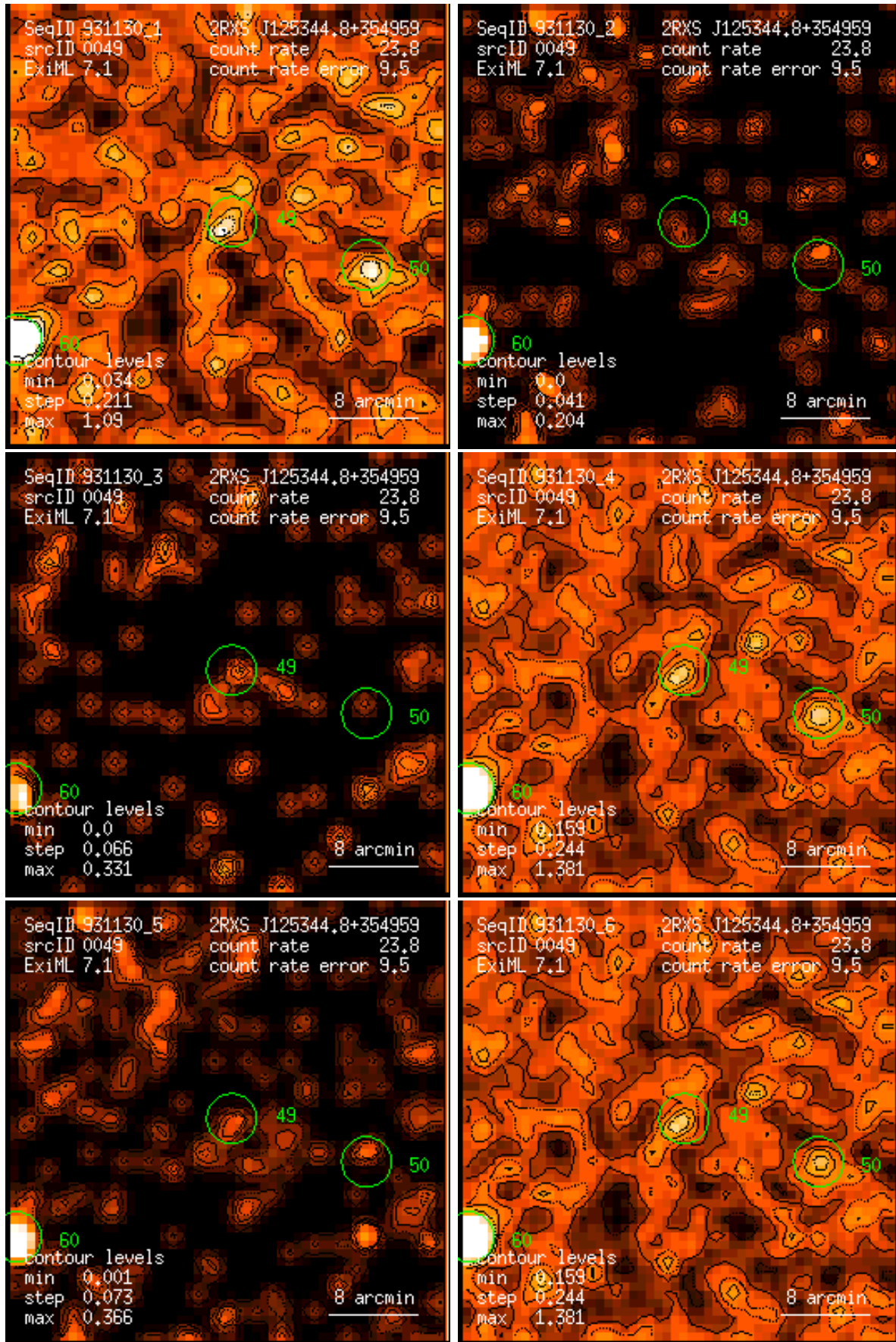
Figure 49: RASS 931130: detection 0049: band rate images, Gaussian filter: (1) PSPC channels 11 – 41, (2) 52 – 90, (3) 91 – 201, (4) 11 – 235, (5) 52 – 201, (6) 11 – 201. Broad band rates in counts/ks. Band rate contour levels in counts/ks/arcmin 2 .
