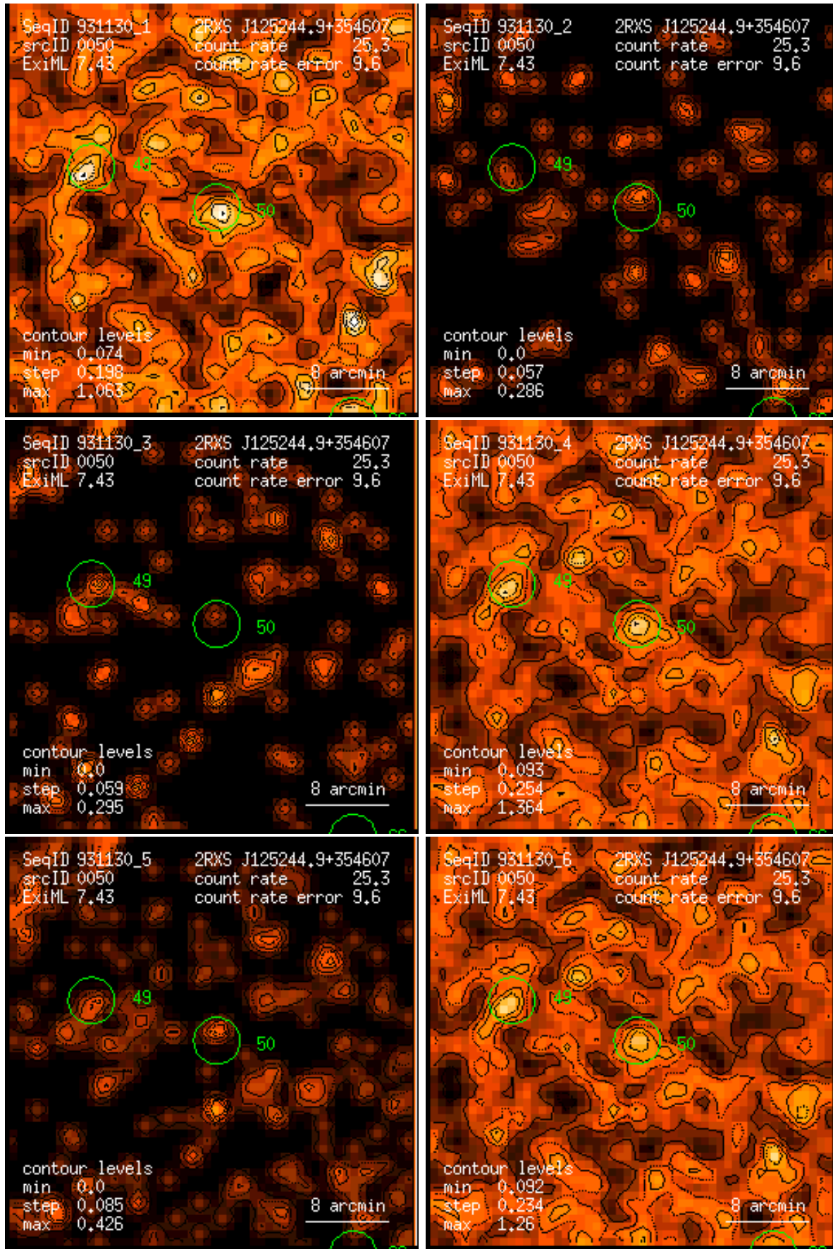
Figure 50: RASS 931130: detection 0050: band rate images, Gaussian filter: (1) PSPC channels 11 – 41, (2) 52 – 90, (3) 91 – 201, (4) 11 – 235, (5) 52 – 201, (6) 11 – 201. Broad band rates in counts/ks. Band rate contour levels in counts/ks/arcmin 2 .
