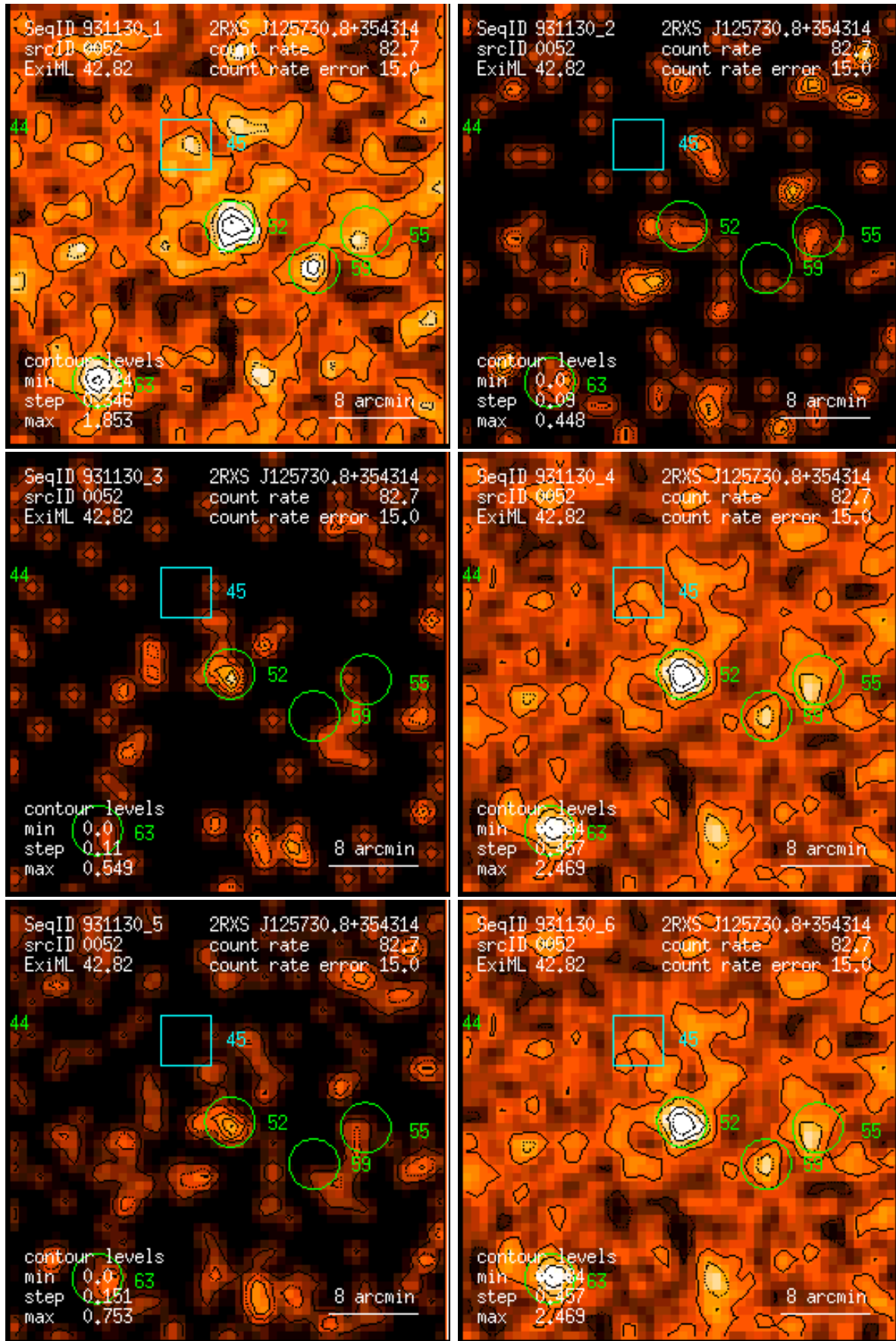
Figure 52: RASS 931130: detection 0052: band rate images, Gaussian filter: (1) PSPC channels 11 – 41, (2) 52 – 90, (3) 91 – 201, (4) 11 – 235, (5) 52 – 201, (6) 11 – 201. Broad band rates in counts/ks. Band rate contour levels in counts/ks/arcmin 2 .
