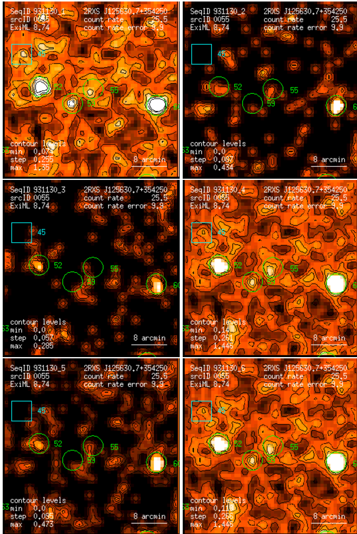
Figure 55: RASS 931130: detection 0055: band rate images, Gaussian filter: (1) PSPC channels 11 – 41, (2) 52 – 90, (3) 91 – 201, (4) 11 – 235, (5) 52 – 201, (6) 11 – 201. Broad band rates in counts/ks. Band rate contour levels in counts/ks/arcmin 2 .
