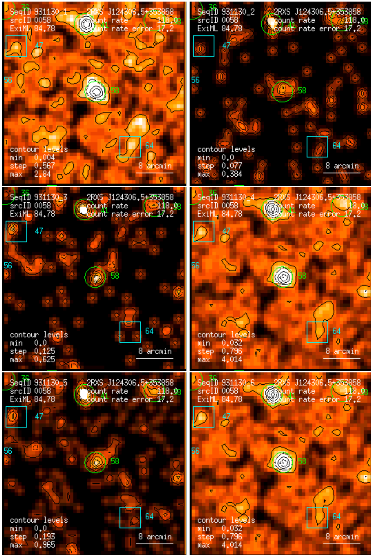
Figure 58: RASS 931130: detection 0058: band rate images, Gaussian filter: (1) PSPC channels 11 – 41, (2) 52 – 90, (3) 91 – 201, (4) 11 – 235, (5) 52 – 201, (6) 11 – 201. Broad band rates in counts/ks. Band rate contour levels in counts/ks/arcmin 2 .
