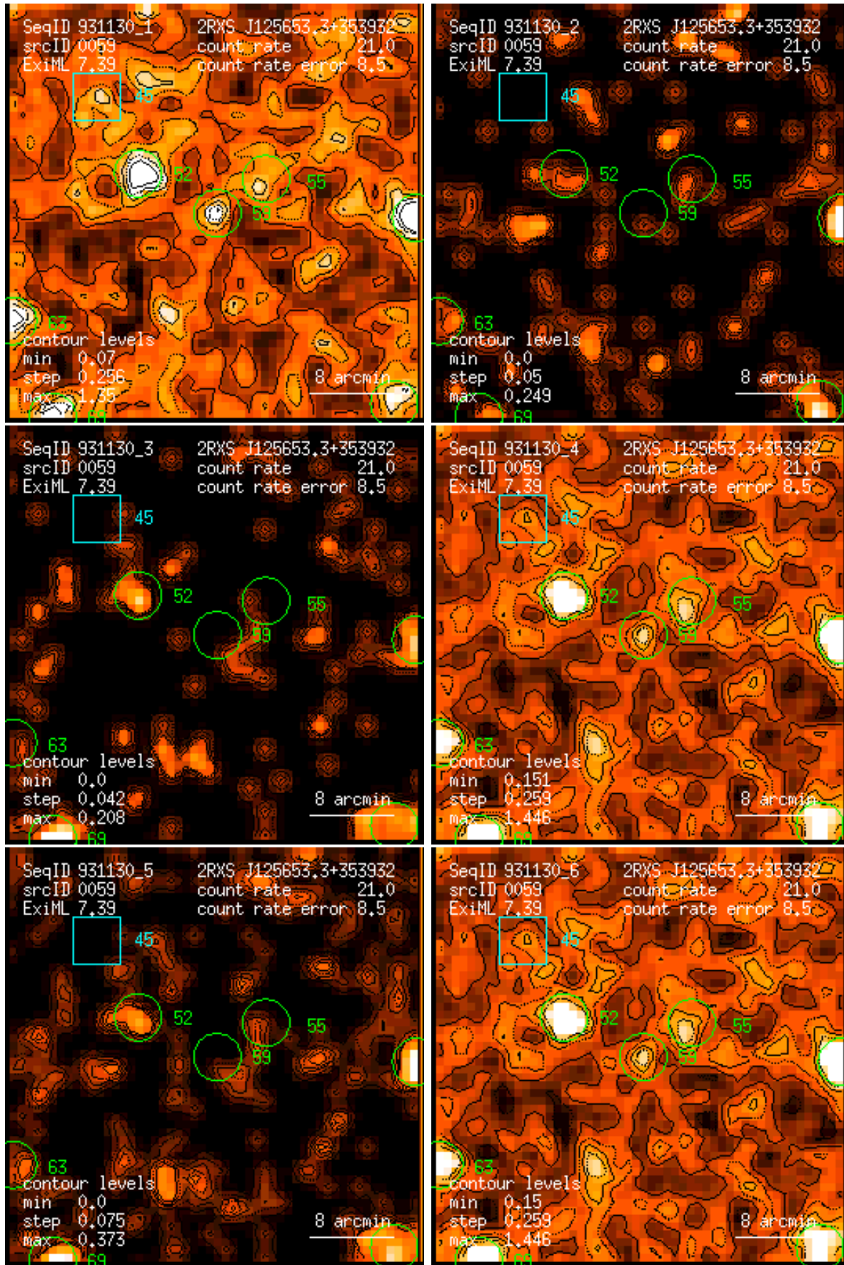
Figure 59: RASS 931130: detection 0059: band rate images, Gaussian filter: (1) PSPC channels 11 – 41, (2) 52 – 90, (3) 91 – 201, (4) 11 – 235, (5) 52 – 201, (6) 11 – 201. Broad band rates in counts/ks. Band rate contour levels in counts/ks/arcmin 2 .
