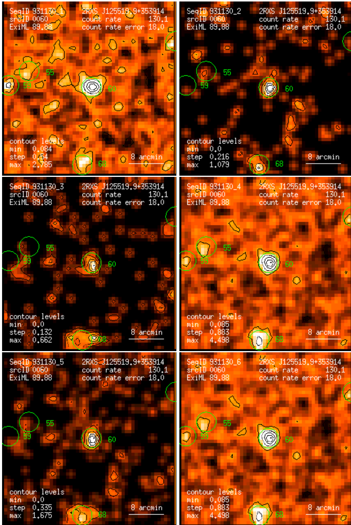
Figure 60: RASS 931130: detection 0060: band rate images, Gaussian filter: (1) PSPC channels 11 – 41, (2) 52 – 90, (3) 91 – 201, (4) 11 – 235, (5) 52 – 201, (6) 11 – 201. Broad band rates in counts/ks. Band rate contour levels in counts/ks/arcmin 2 .
