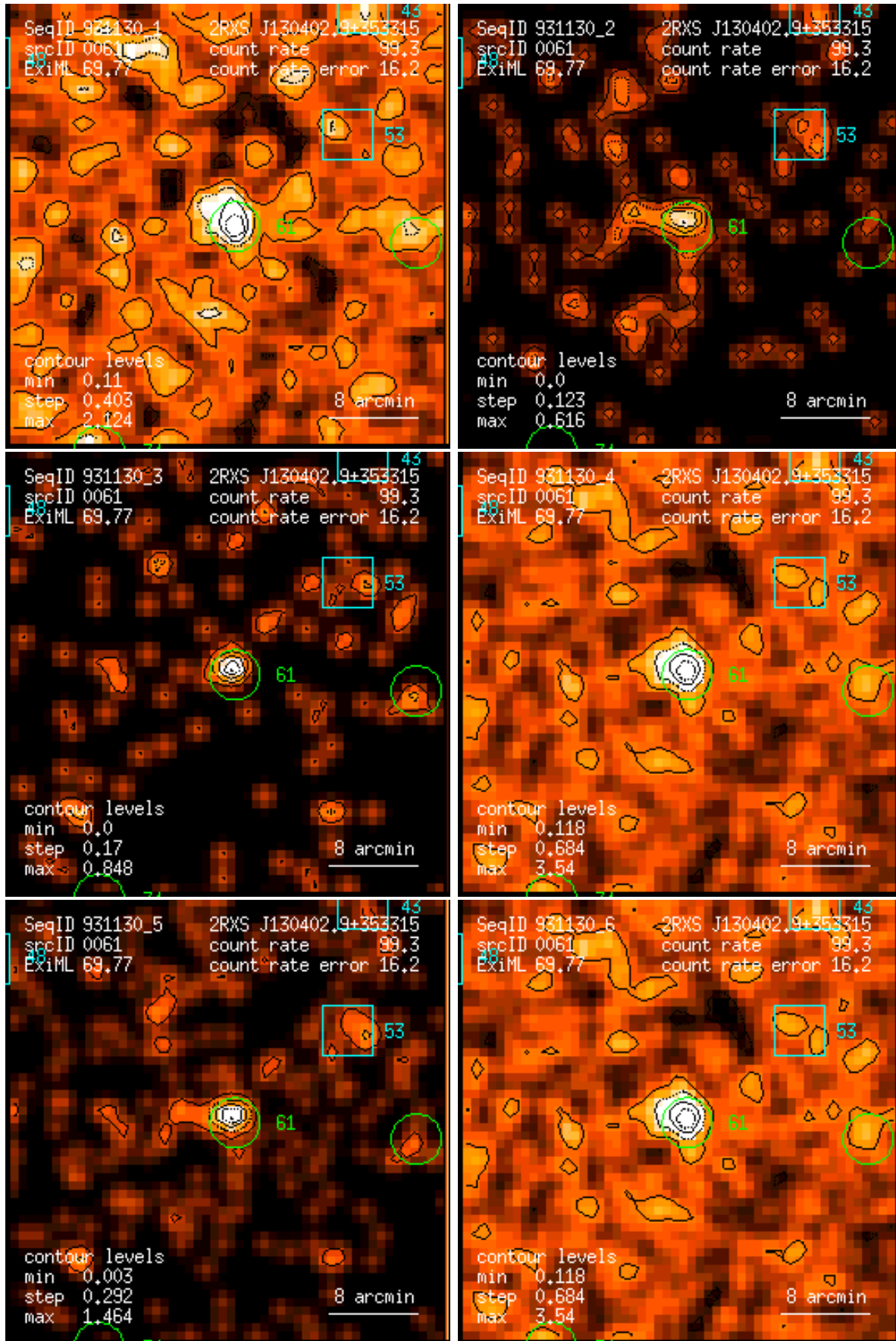
Figure 61: RASS 931130: detection 0061: band rate images, Gaussian filter: (1) PSPC channels 11 – 41, (2) 52 – 90, (3) 91 – 201, (4) 11 – 235, (5) 52 – 201, (6) 11 – 201. Broad band rates in counts/ks. Band rate contour levels in counts/ks/arcmin 2 .
