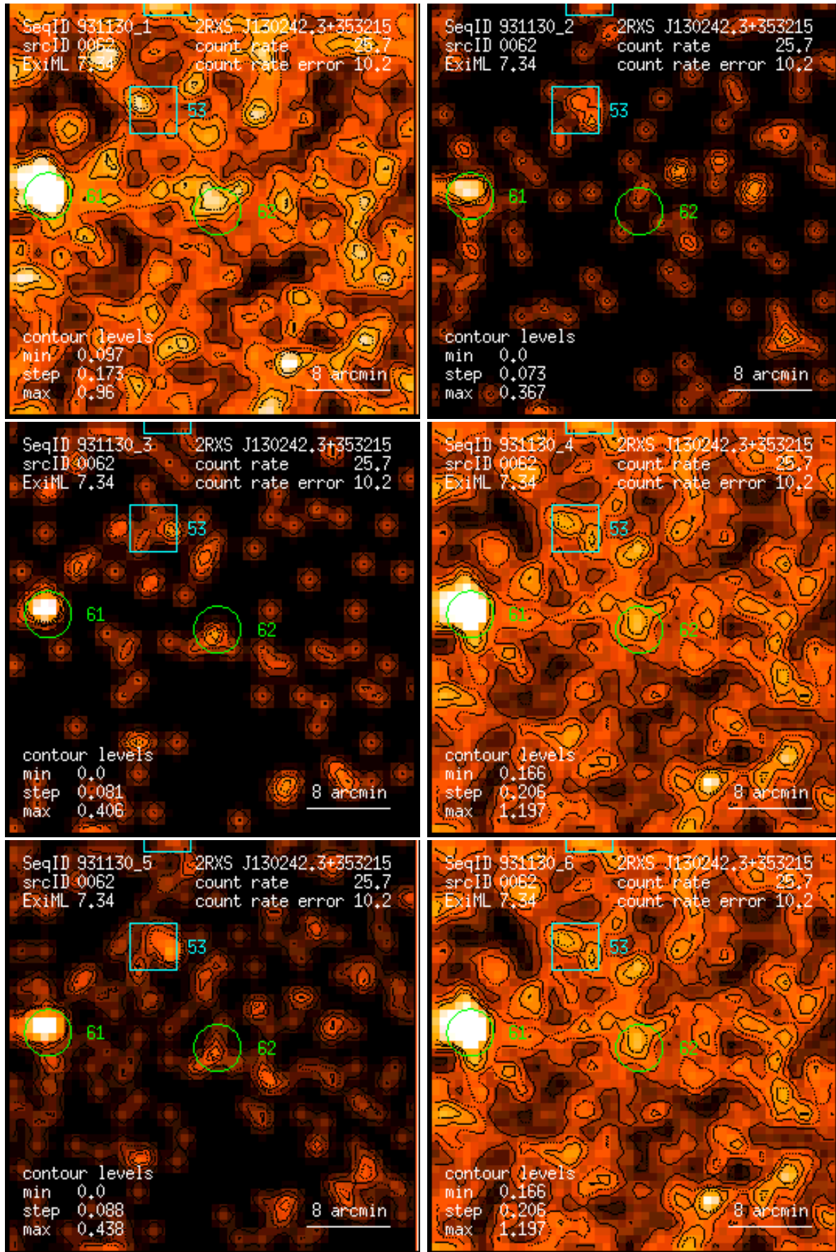
Figure 62: RASS 931130: detection 0062: band rate images, Gaussian filter: (1) PSPC channels 11 – 41, (2) 52 – 90, (3) 91 – 201, (4) 11 – 235, (5) 52 – 201, (6) 11 – 201. Broad band rates in counts/ks. Band rate contour levels in counts/ks/arcmin 2 .
