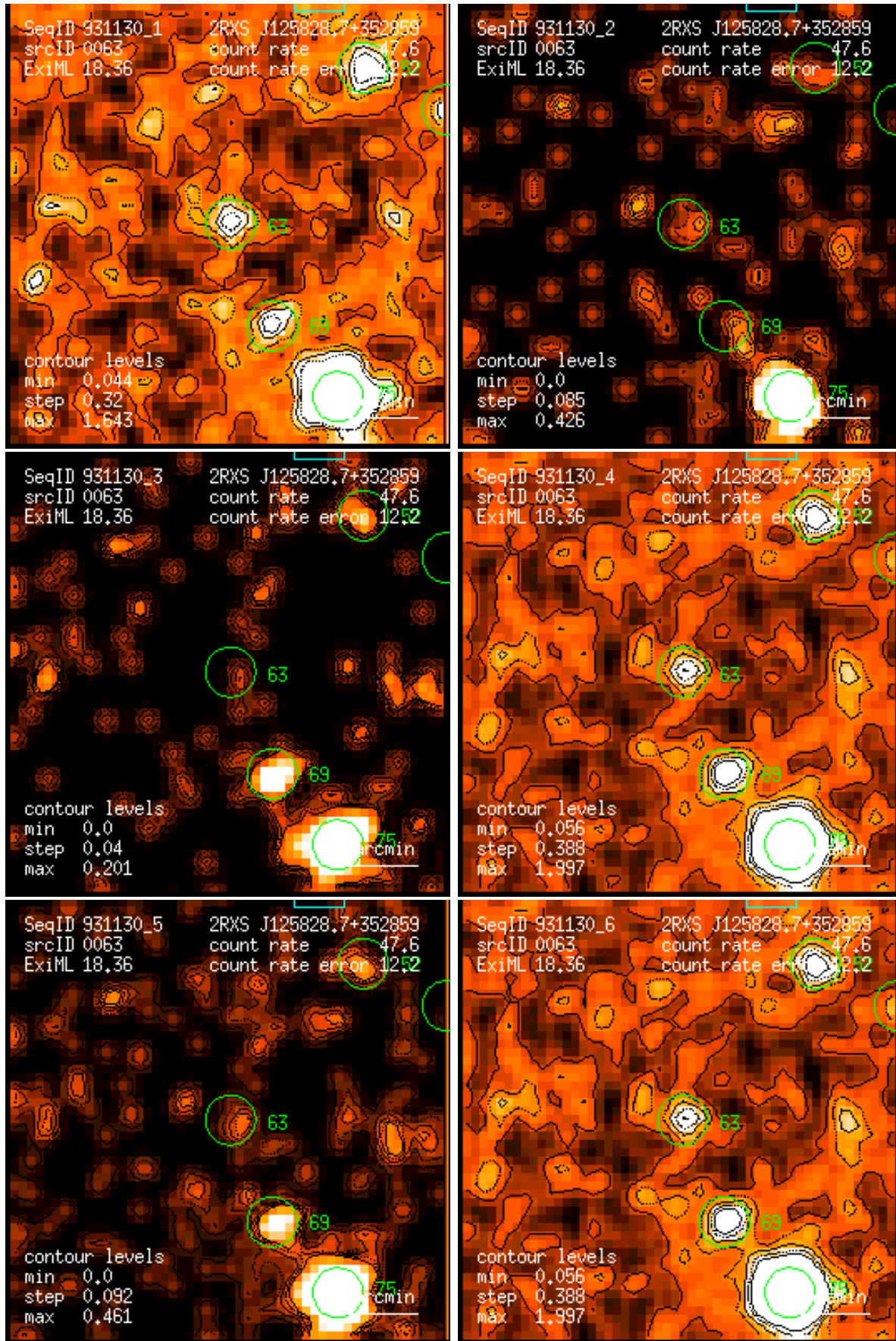
Figure 63: RASS 931130: detection 0063: band rate images, Gaussian filter: (1) PSPC channels 11 – 41, (2) 52 – 90, (3) 91 – 201, (4) 11 – 235, (5) 52 – 201, (6) 11 – 201. Broad band rates in counts/ks. Band rate contour levels in counts/ks/arcmin 2 .
