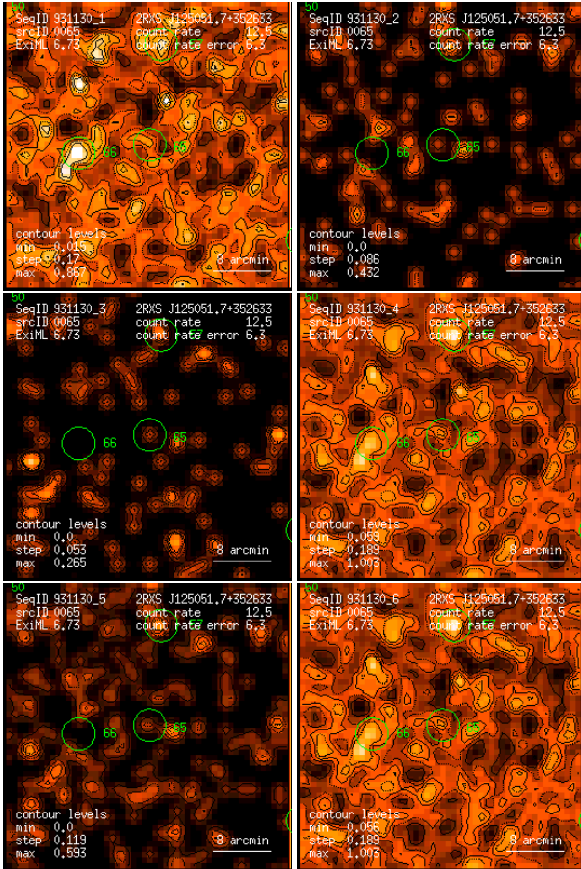
Figure 65: RASS 931130: detection 0065: band rate images, Gaussian filter: (1) PSPC channels 11 – 41, (2) 52 – 90, (3) 91 – 201, (4) 11 – 235, (5) 52 – 201, (6) 11 – 201. Broad band rates in counts/ks. Band rate contour levels in counts/ks/arcmin 2 .
