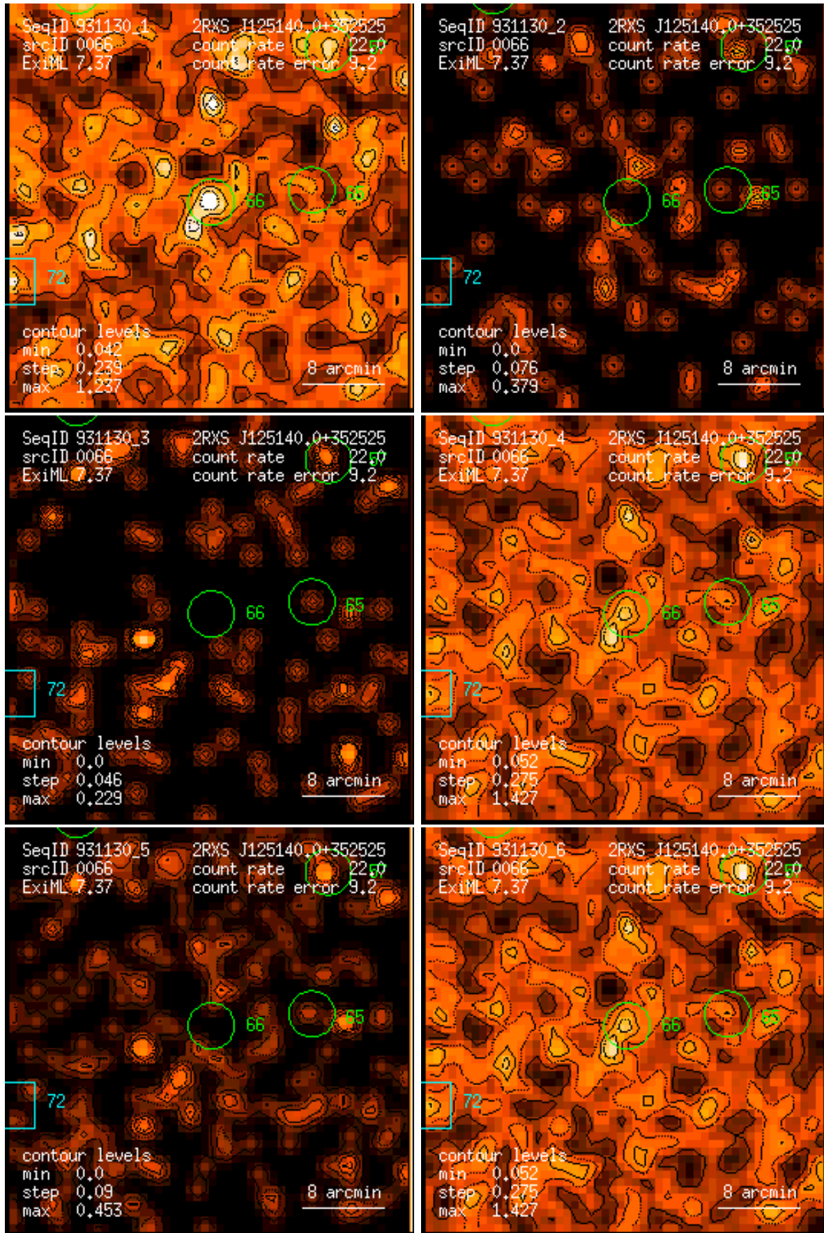
Figure 66: RASS 931130: detection 0066: band rate images, Gaussian filter: (1) PSPC channels 11 – 41, (2) 52 – 90, (3) 91 – 201, (4) 11 – 235, (5) 52 – 201, (6) 11 – 201. Broad band rates in counts/ks. Band rate contour levels in counts/ks/arcmin 2 .
