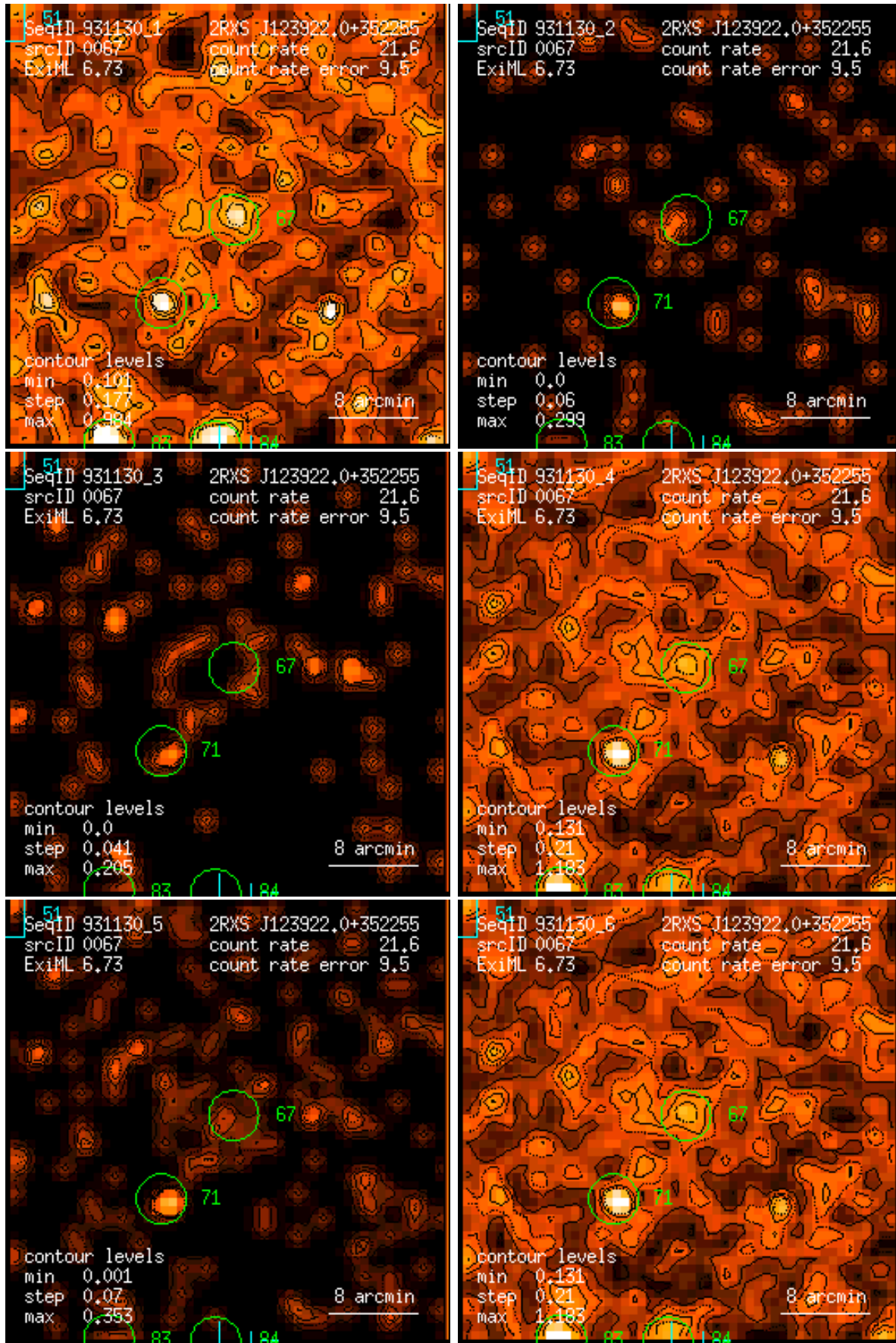
Figure 67: RASS 931130: detection 0067: band rate images, Gaussian filter: (1) PSPC channels 11 – 41, (2) 52 – 90, (3) 91 – 201, (4) 11 – 235, (5) 52 – 201, (6) 11 – 201. Broad band rates in counts/ks. Band rate contour levels in counts/ks/arcmin 2 .
