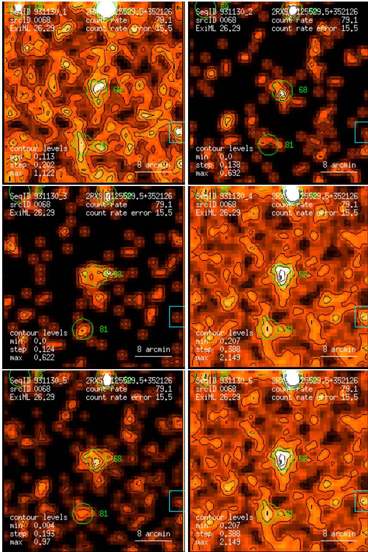
Figure 68: RASS 931130: detection 0068: band rate images, Gaussian filter: (1) PSPC channels 11 – 41, (2) 52 – 90, (3) 91 – 201, (4) 11 – 235, (5) 52 – 201, (6) 11 – 201. Broad band rates in counts/ks. Band rate contour levels in counts/ks/arcmin 2 .
