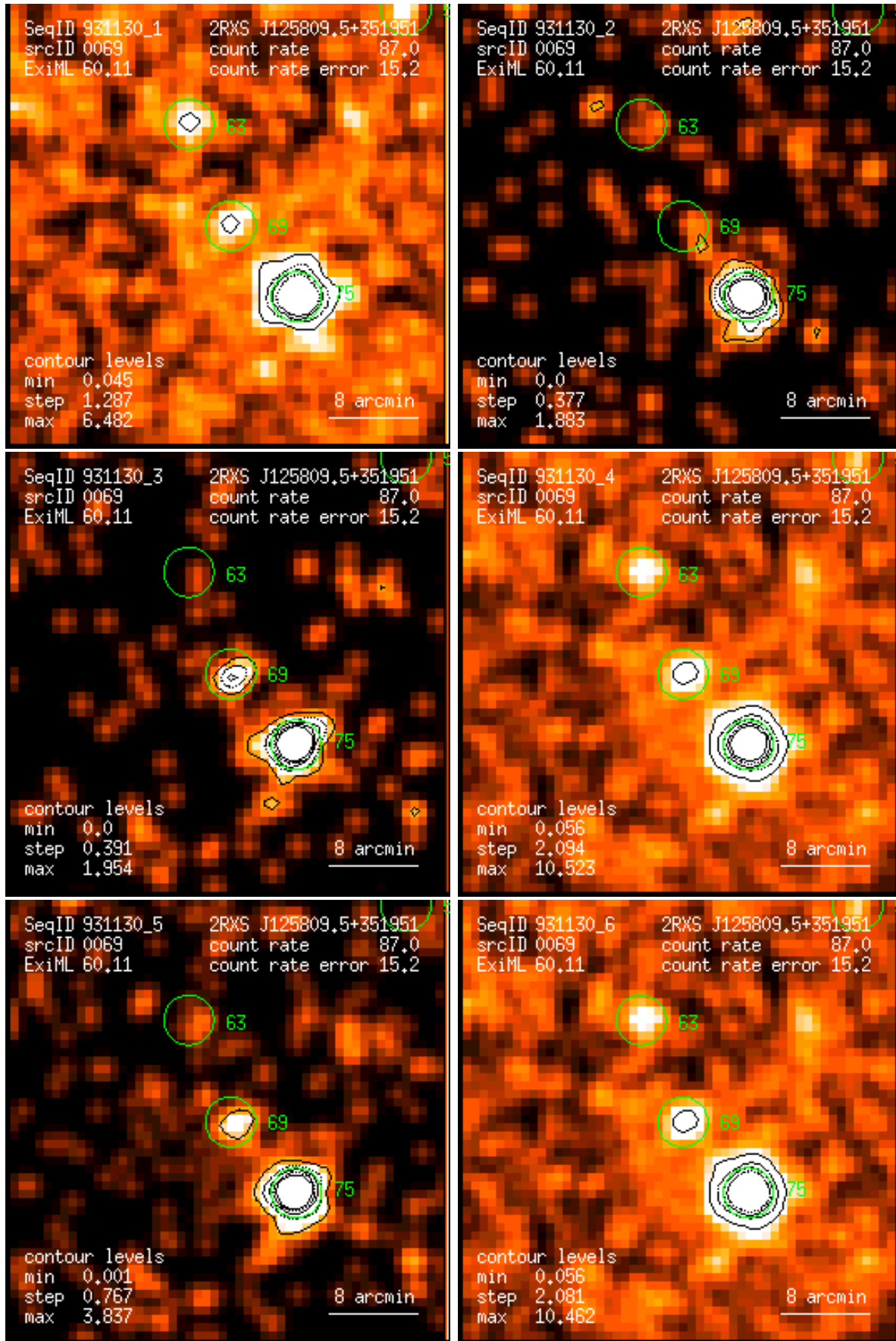
Figure 69: RASS 931130: detection 0069: band rate images, Gaussian filter: (1) PSPC channels 11 – 41, (2) 52 – 90, (3) 91 – 201, (4) 11 – 235, (5) 52 – 201, (6) 11 – 201. Broad band rates in counts/ks. Band rate contour levels in counts/ks/arcmin 2 .
