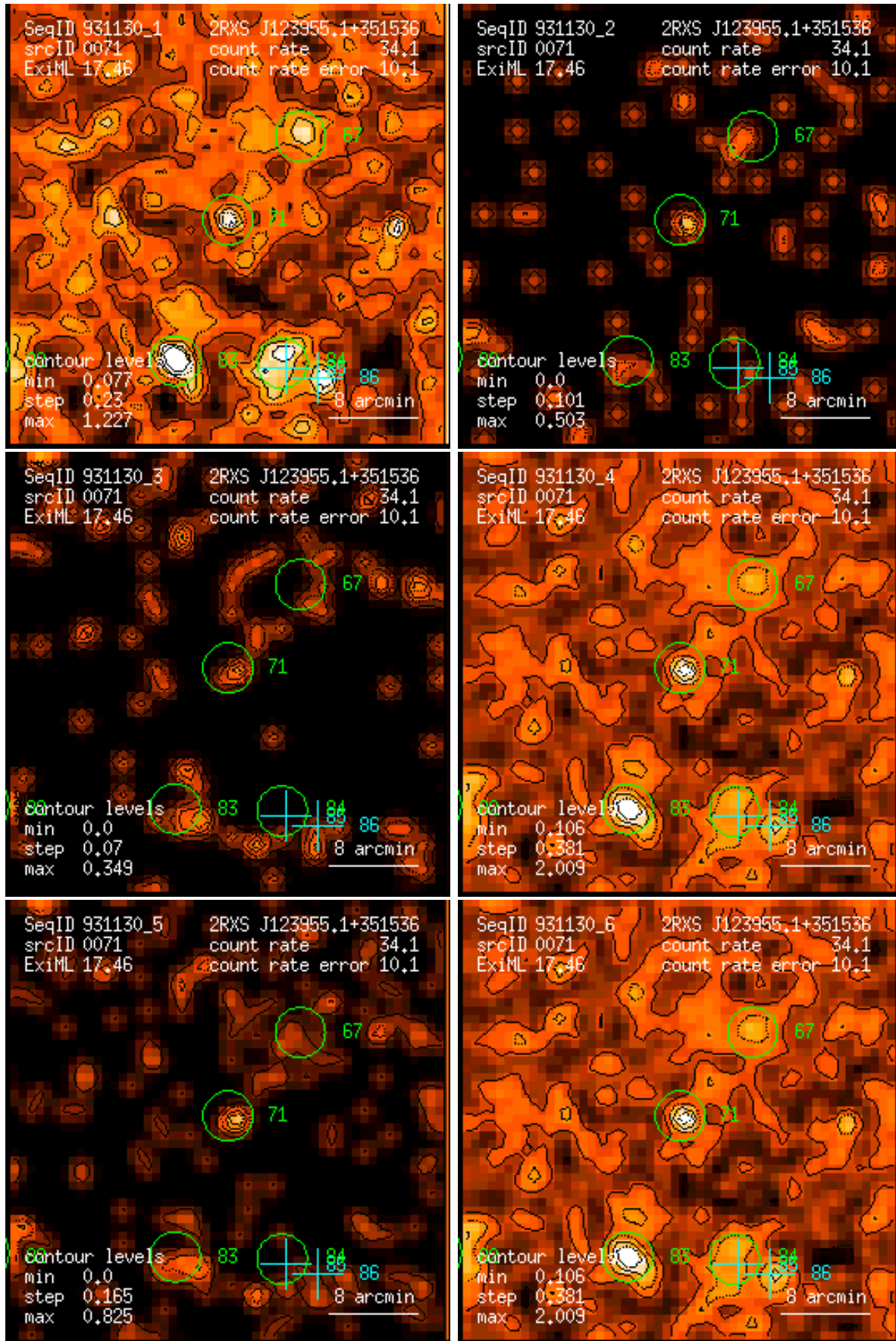
Figure 71: RASS 931130: detection 0071: band rate images, Gaussian filter: (1) PSPC channels 11 – 41, (2) 52 – 90, (3) 91 – 201, (4) 11 – 235, (5) 52 – 201, (6) 11 – 201. Broad band rates in counts/ks. Band rate contour levels in counts/ks/arcmin 2 .
