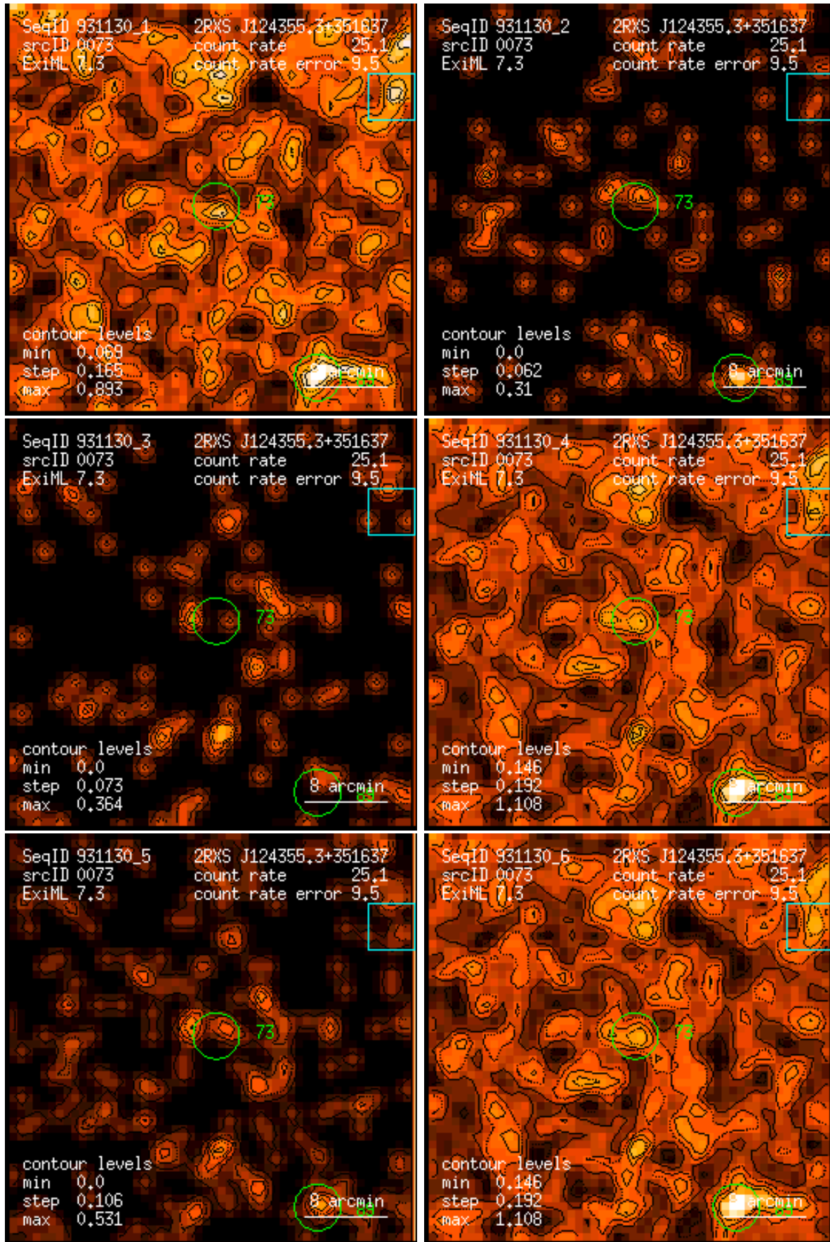
Figure 73: RASS 931130: detection 0073: band rate images, Gaussian filter: (1) PSPC channels 11 – 41, (2) 52 – 90, (3) 91 – 201, (4) 11 – 235, (5) 52 – 201, (6) 11 – 201. Broad band rates in counts/ks. Band rate contour levels in counts/ks/arcmin 2 .
