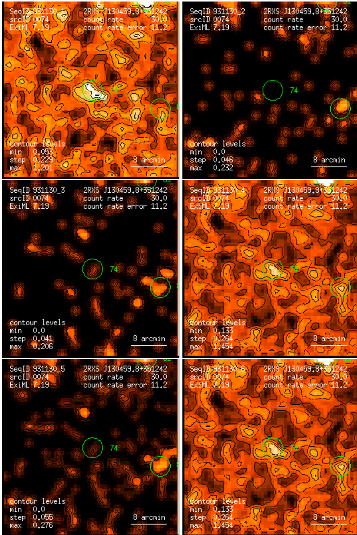
Figure 74: RASS 931130: detection 0074: band rate images, Gaussian filter: (1) PSPC channels 11 – 41, (2) 52 – 90, (3) 91 – 201, (4) 11 – 235, (5) 52 – 201, (6) 11 – 201. Broad band rates in counts/ks. Band rate contour levels in counts/ks/arcmin 2 .
