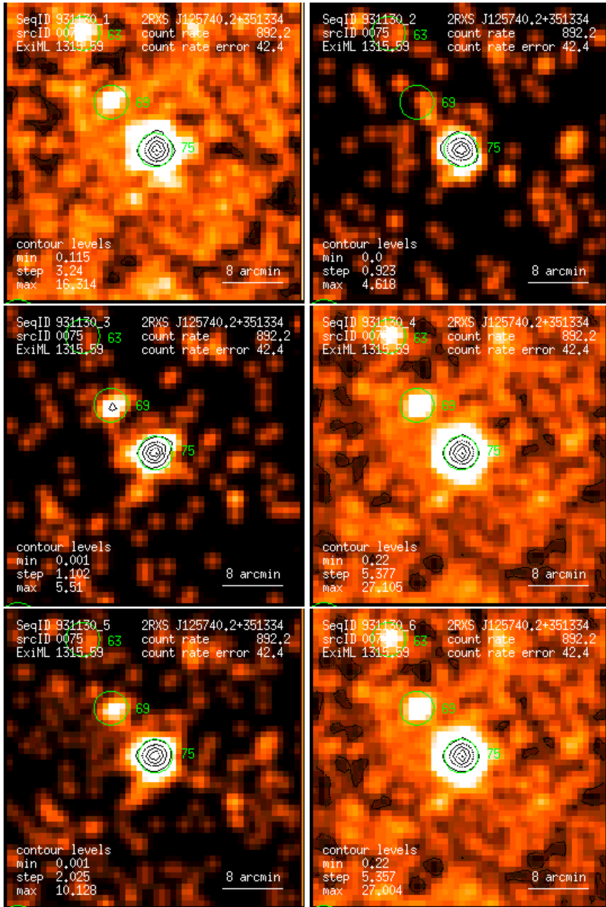
Figure 75: RASS 931130: detection 0075: band rate images, Gaussian filter: (1) PSPC channels 11 – 41, (2) 52 – 90, (3) 91 – 201, (4) 11 – 235, (5) 52 – 201, (6) 11 – 201. Broad band rates in counts/ks. Band rate contour levels in counts/ks/arcmin 2 .
