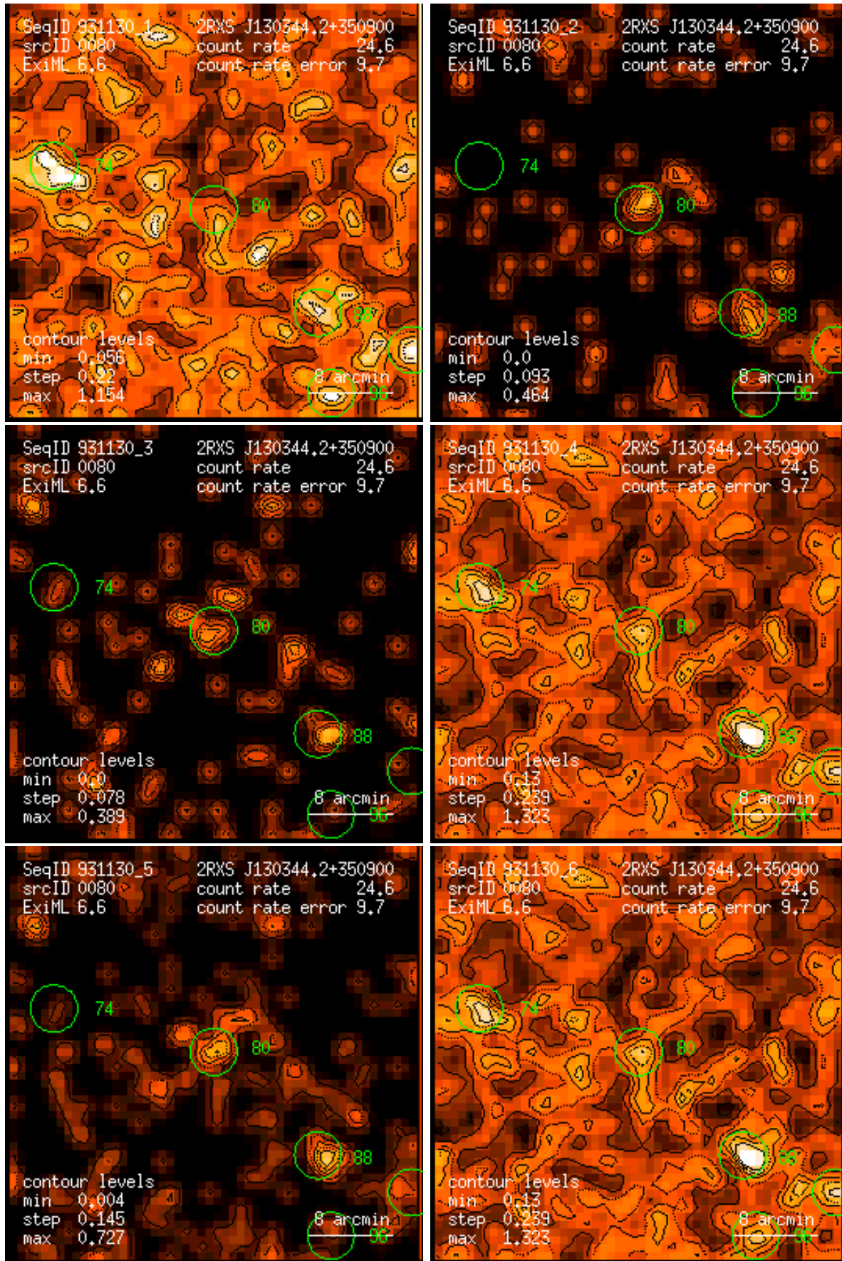
Figure 80: RASS 931130: detection 0080: band rate images, Gaussian filter: (1) PSPC channels 11 – 41, (2) 52 – 90, (3) 91 – 201, (4) 11 – 235, (5) 52 – 201, (6) 11 – 201. Broad band rates in counts/ks. Band rate contour levels in counts/ks/arcmin 2 .
