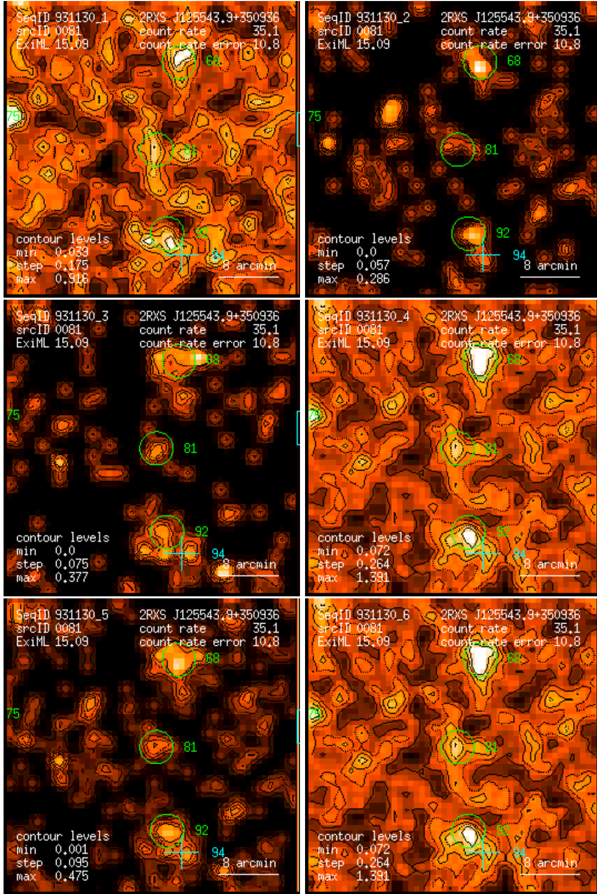
Figure 81: RASS 931130: detection 0081: band rate images, Gaussian filter: (1) PSPC channels 11 – 41, (2) 52 – 90, (3) 91 – 201, (4) 11 – 235, (5) 52 – 201, (6) 11 – 201. Broad band rates in counts/ks. Band rate contour levels in counts/ks/arcmin 2 .
