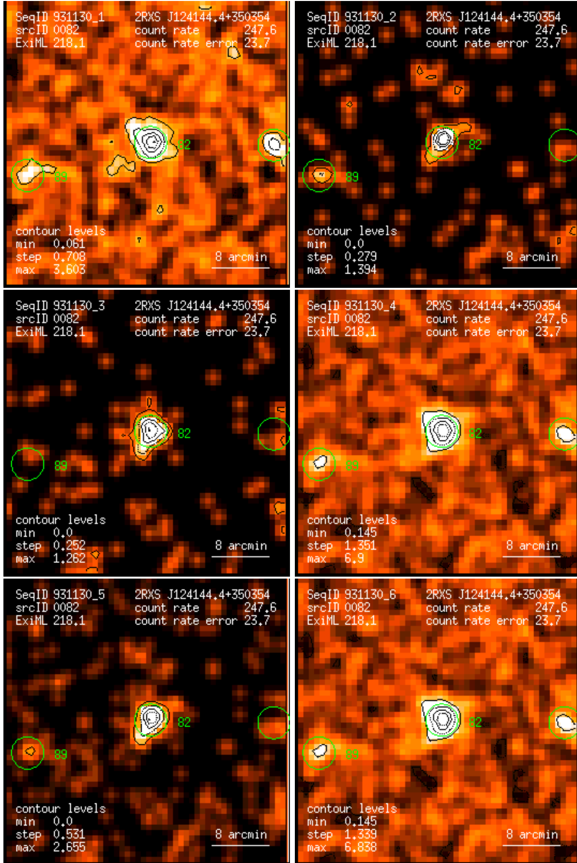
Figure 82: RASS 931130: detection 0082: band rate images, Gaussian filter: (1) PSPC channels 11 – 41, (2) 52 – 90, (3) 91 – 201, (4) 11 – 235, (5) 52 – 201, (6) 11 – 201. Broad band rates in counts/ks. Band rate contour levels in counts/ks/arcmin 2 .
