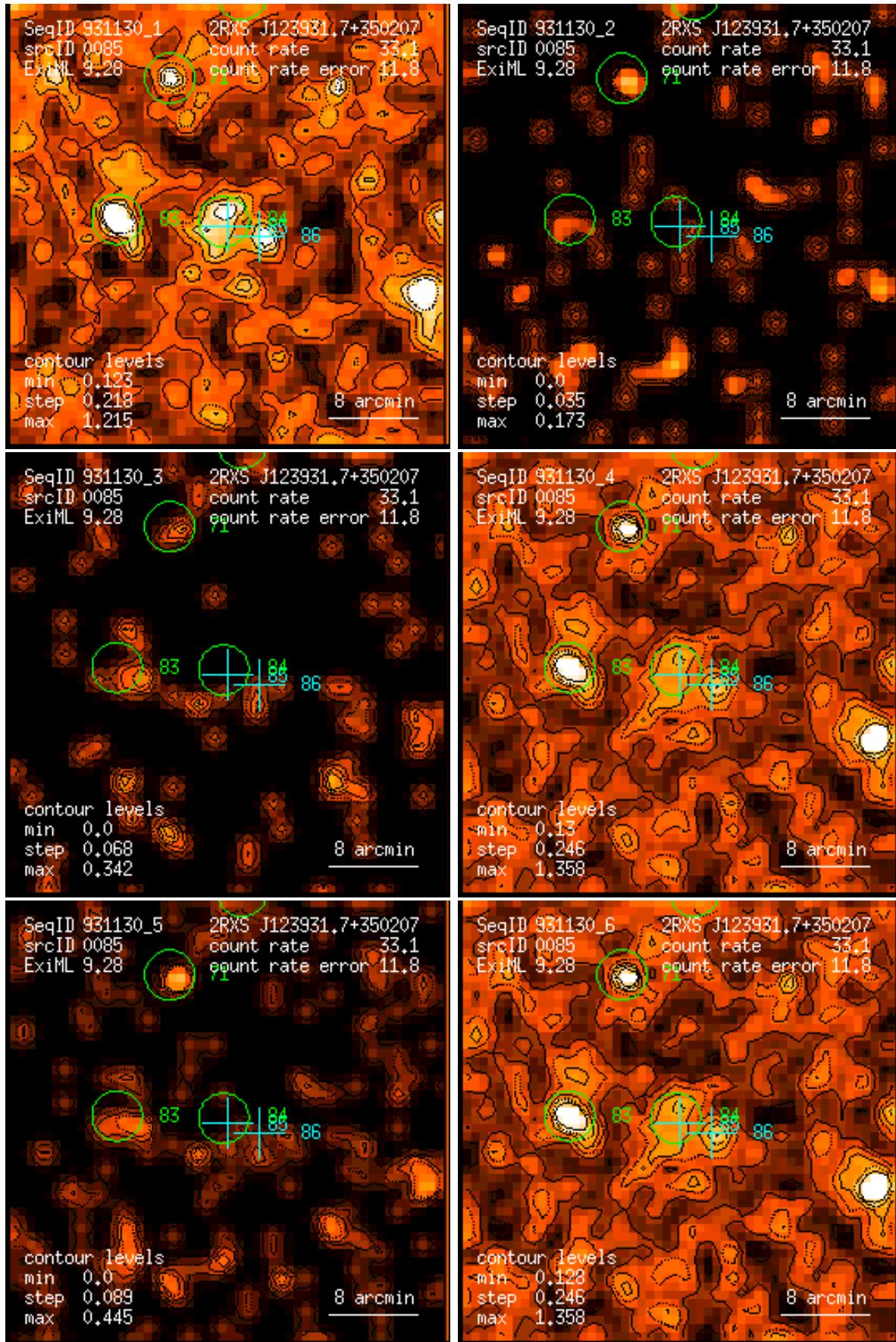
Figure 85: RASS 931130: detection 0085: band rate images, Gaussian filter: (1) PSPC channels 11 – 41, (2) 52 – 90, (3) 91 – 201, (4) 11 – 235, (5) 52 – 201, (6) 11 – 201. Broad band rates in counts/ks. Band rate contour levels in counts/ks/arcmin 2 .
