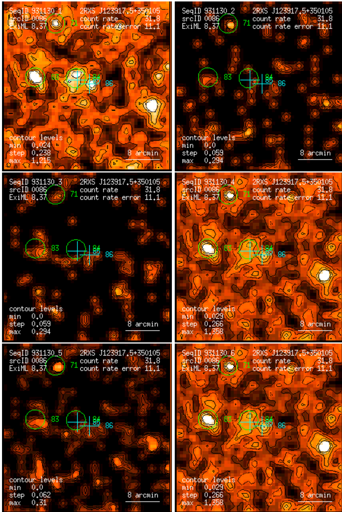
Figure 86: RASS 931130: detection 0086: band rate images, Gaussian filter: (1) PSPC channels 11 – 41, (2) 52 – 90, (3) 91 – 201, (4) 11 – 235, (5) 52 – 201, (6) 11 – 201. Broad band rates in counts/ks. Band rate contour levels in counts/ks/arcmin 2 .
