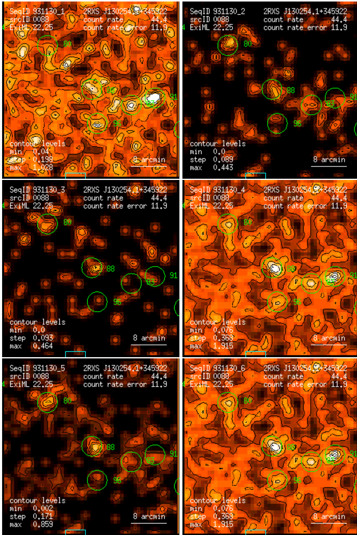
Figure 88: RASS 931130: detection 0088: band rate images, Gaussian filter: (1) PSPC channels 11 – 41, (2) 52 – 90, (3) 91 – 201, (4) 11 – 235, (5) 52 – 201, (6) 11 – 201. Broad band rates in counts/ks. Band rate contour levels in counts/ks/arcmin 2 .
