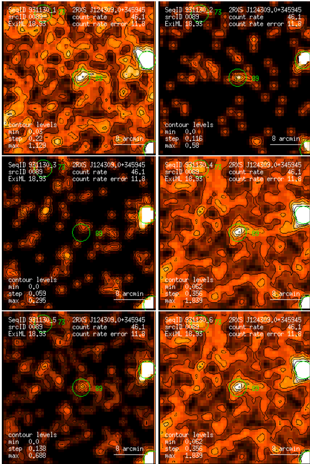
Figure 89: RASS 931130: detection 0089: band rate images, Gaussian filter: (1) PSPC channels 11 – 41, (2) 52 – 90, (3) 91 – 201, (4) 11 – 235, (5) 52 – 201, (6) 11 – 201. Broad band rates in counts/ks. Band rate contour levels in counts/ks/arcmin 2 .
