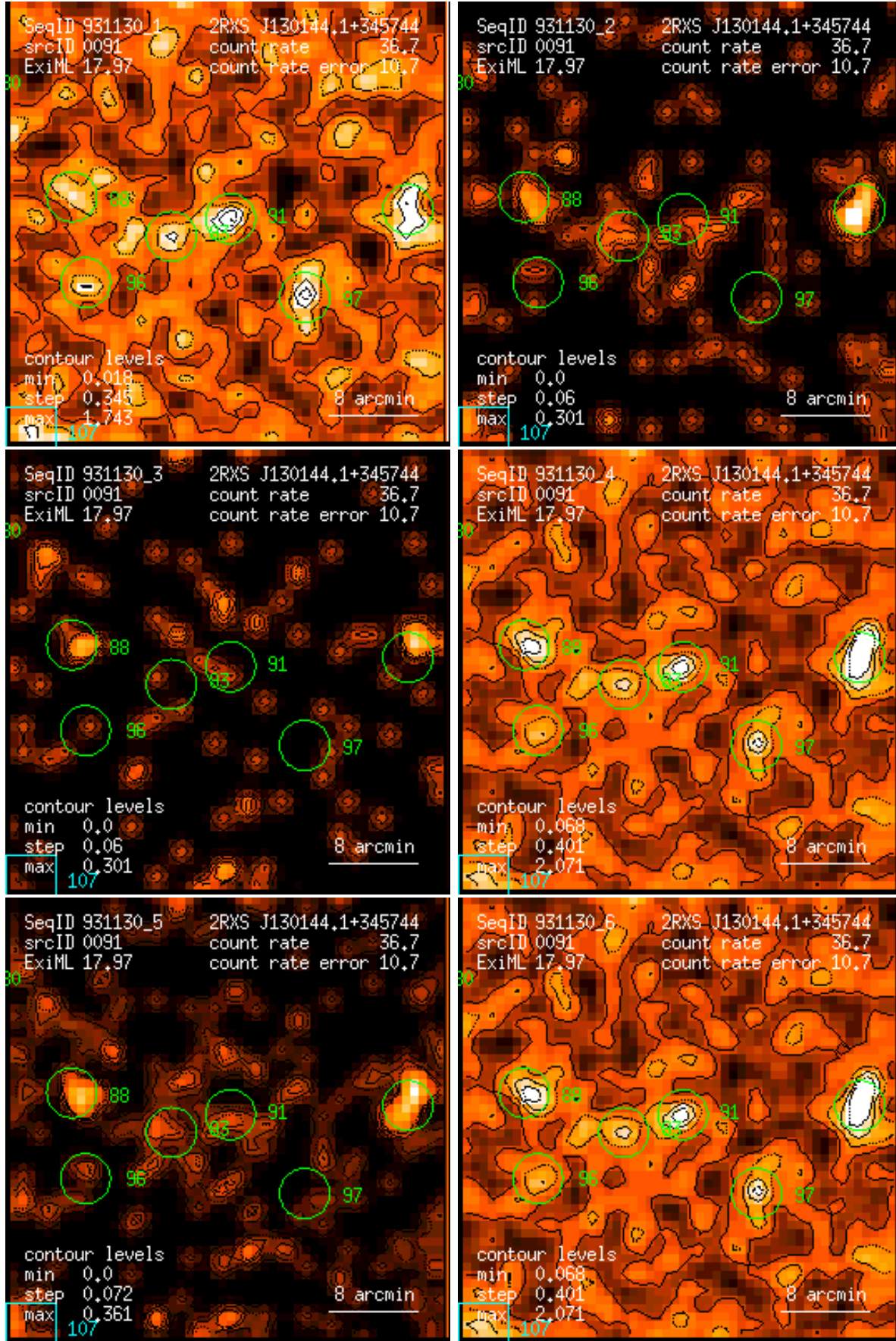
Figure 91: RASS 931130: detection 0091: band rate images, Gaussian filter: (1) PSPC channels 11 – 41, (2) 52 – 90, (3) 91 – 201, (4) 11 – 235, (5) 52 – 201, (6) 11 – 201. Broad band rates in counts/ks. Band rate contour levels in counts/ks/arcmin 2 .
